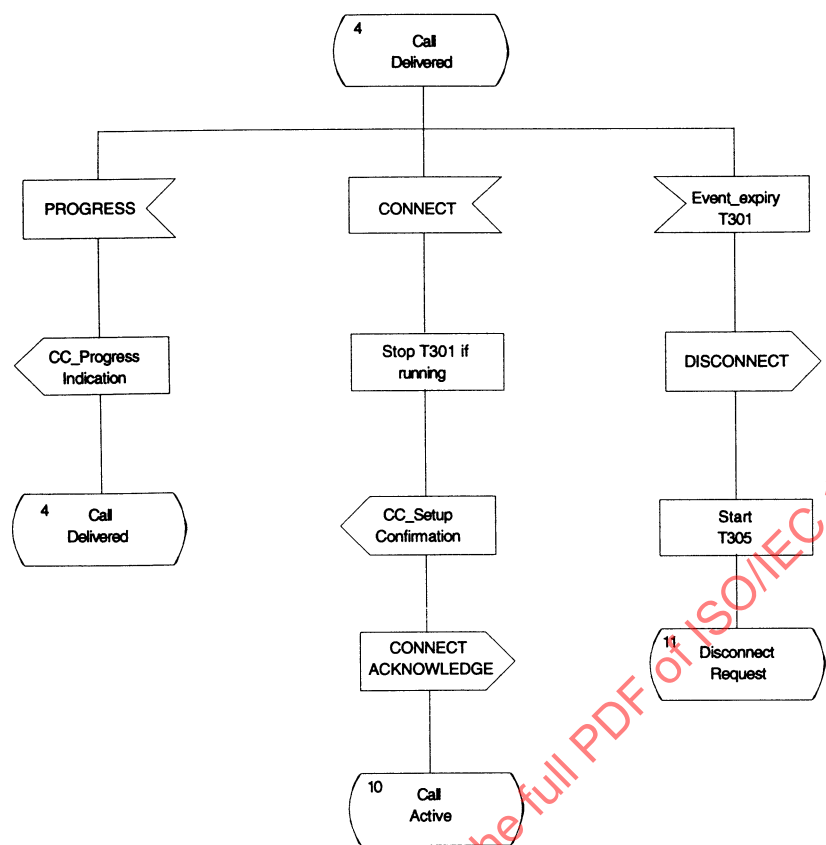
Figure E.2 — Protocol Control SDL diagram (sheet 8 of 22) (continued)
