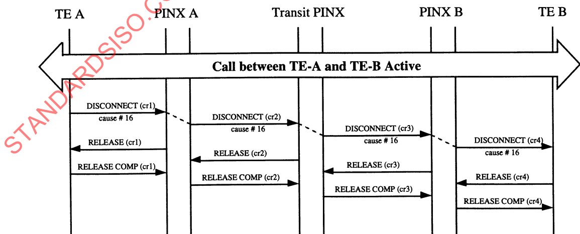
Figure C.5 — Normal call clearing by originator
