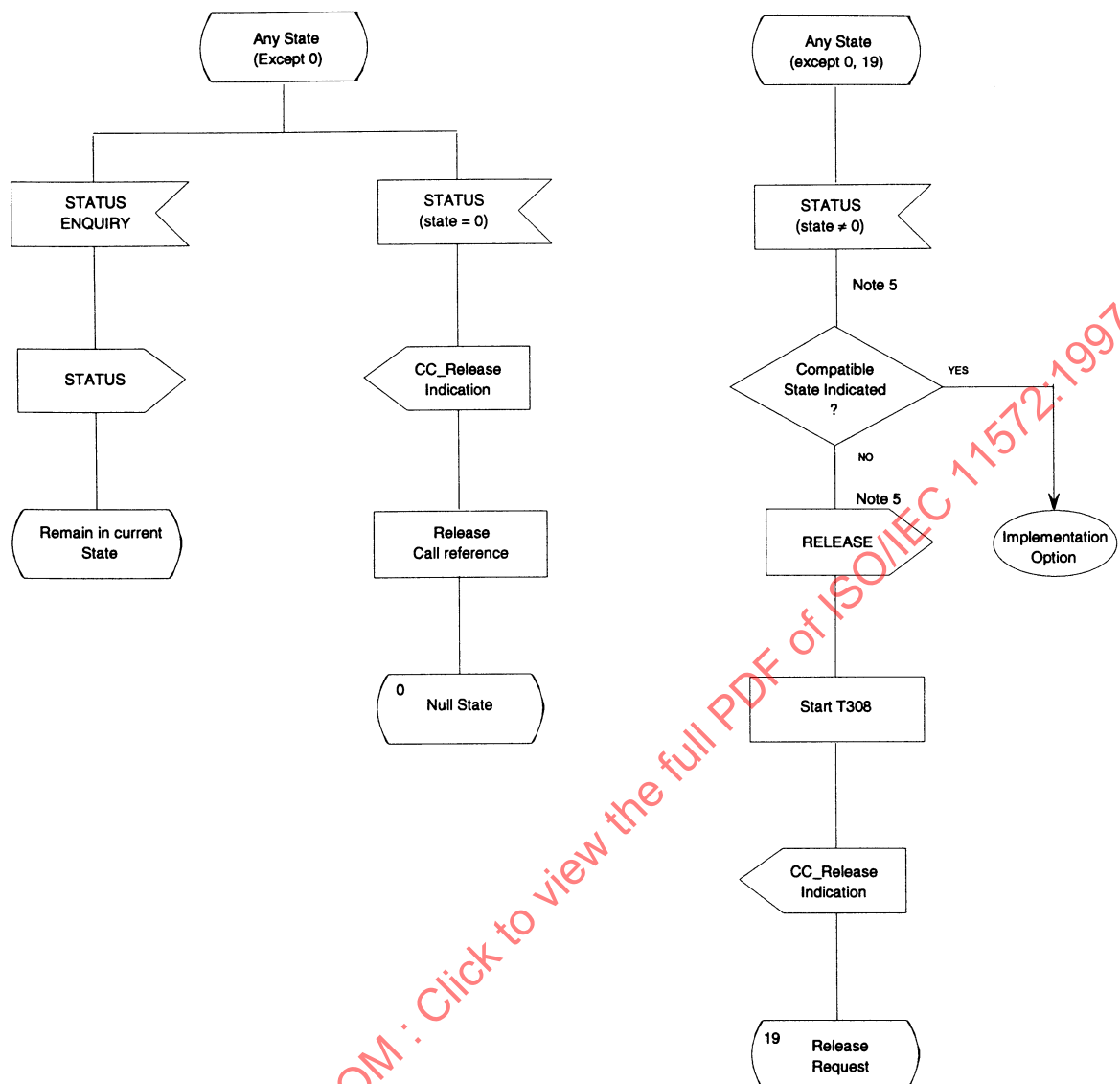
Figure E.2 — Protocol Control SDL diagram (sheet 17 of 22) (continued)
