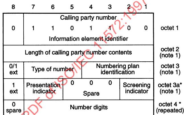
Figure 17 — Calling party number information element
