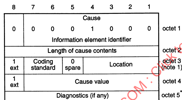
Figure 18 — Cause information element
