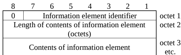
Figure 11 - Variable length information element format
