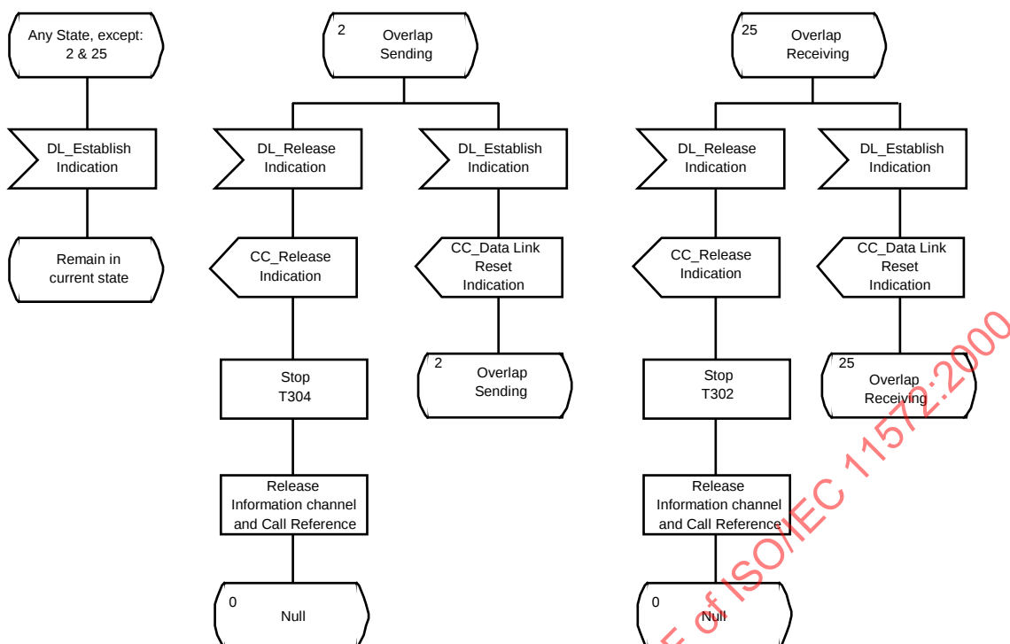
Figure E.2 - Protocol Control SDL diagram (sheet 21 of 22) (continued)
