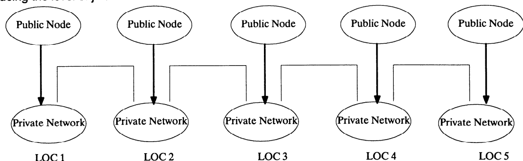
Figure A.2 – Private Digital Network Synchronization Reference at Each Interface with a carrier
