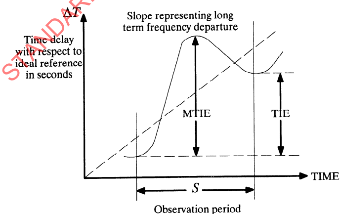
Figure 1 – Time Interval Error (TIE)
