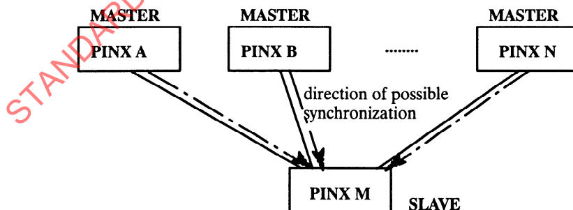
Figure B.3 – Multiple Master – Slave Configuration
