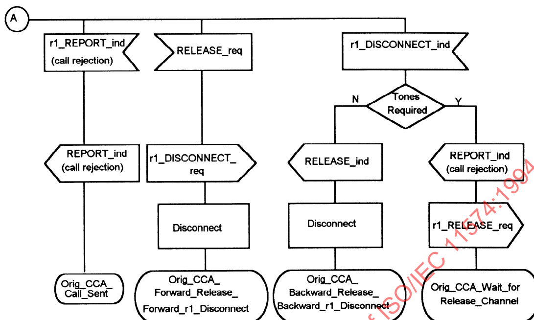
Figure 19 – Stage 2 SDL diagram for Originating CCA functional entity (Sheet 4 of 9)
