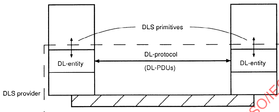
Figure 2 — Structure of DLS provider
