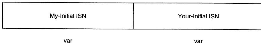
Figure 13-12 – Enciphered Auth-data
