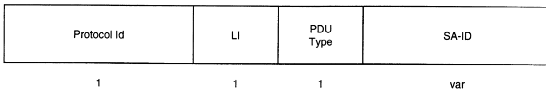
Figure 13-4 – Unprotected Header
