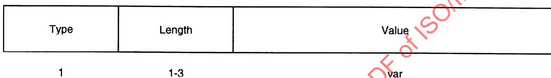
Figure 13-1 – Content Field
