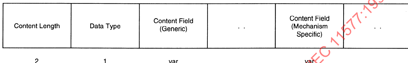
Figure 13-6 – Octet-String-Before-Encapsulation
