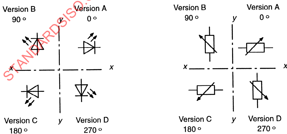
Figure 15 – Possible versions of composite graphical symbols
