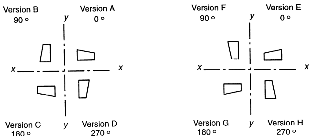
Figure 13 – Possible versions of the graphical symbol for an asymmetric reduction
