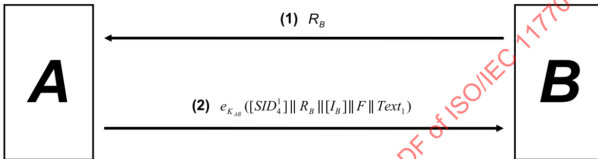
Figure 4 — Mechanism 4
