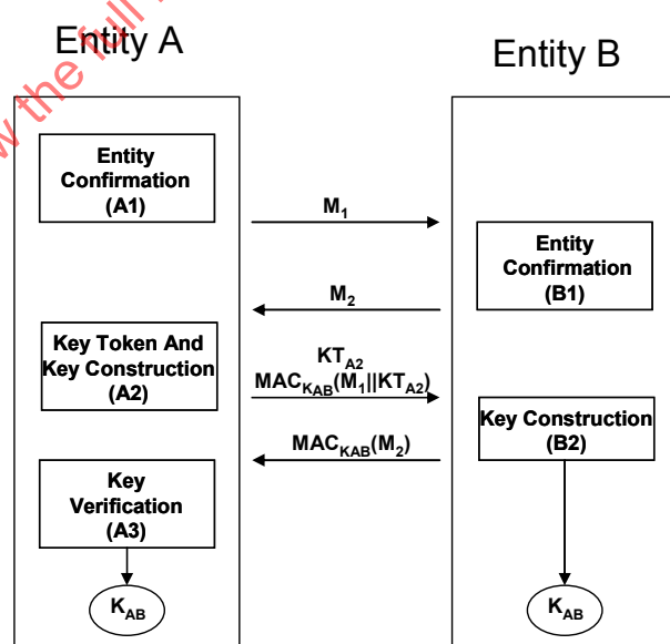
Figure 8: Key Agreement Mechanism 11
