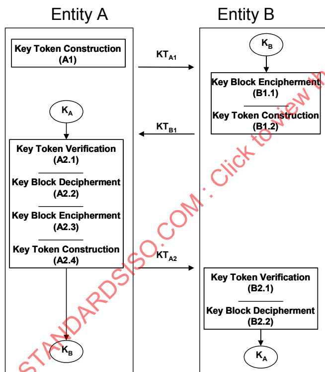
Figure 13: Key Transport Mechanism 5
