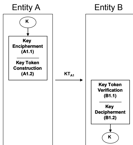
Figure 10: Key Transport Mechanism 2
