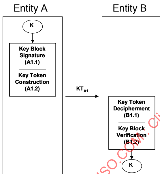
Figure 11: Key Transport Mechanism 3
