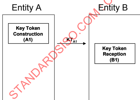
Figure 15: Public Key Transport Mechanism 1
