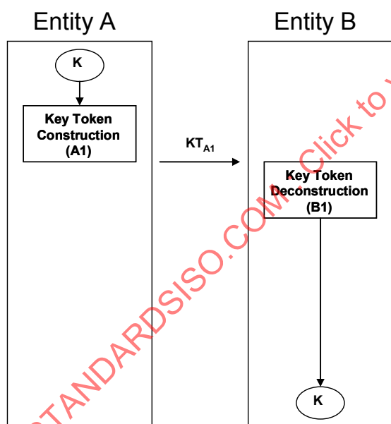
Figure 9: Key Transport Mechanism 1
