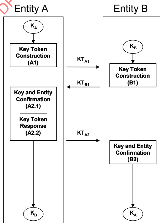
Figure 14: Key Transport Mechanism 6
