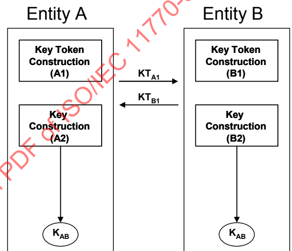
Figure 4: Key Agreement Mechanisms 4, 5, 9
