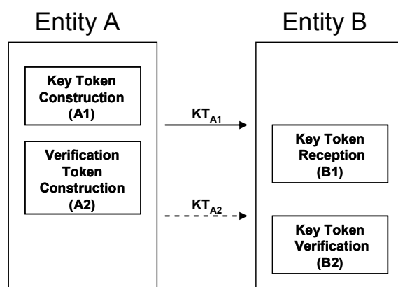
Figure 16: Public Key Transport Mechanism 2
