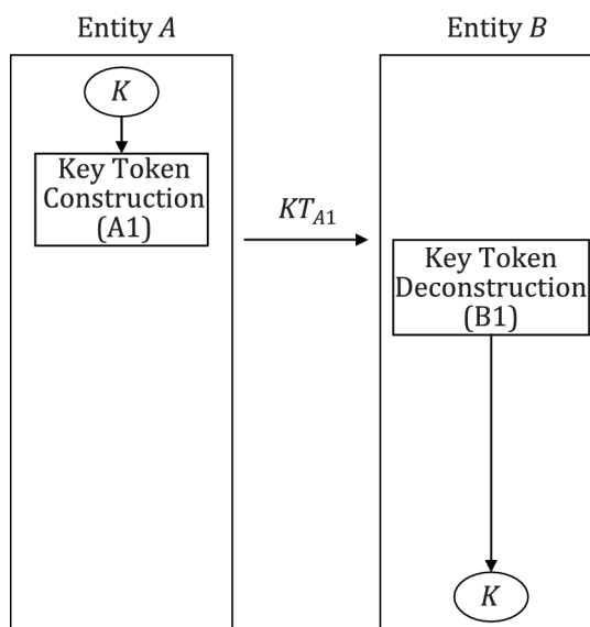
Figure 13 — Secret key transport mechanism 1
