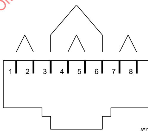
Figure 9 – Pin grouping and pair assignments for IEC 60603-7 series interface for Categories 5, 6, 6 A and 8.1 (front view of fixed connector (jack), not to scale)
