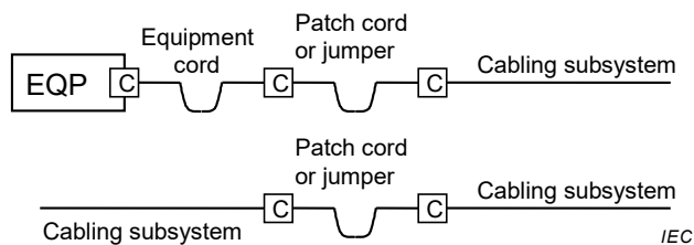
Figure 4 – Cross-connect models
