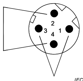
Figure 12 – Four position connector pin and pair assignments for IEC 61076-2-101 connecting hardware (front view of male connector)
