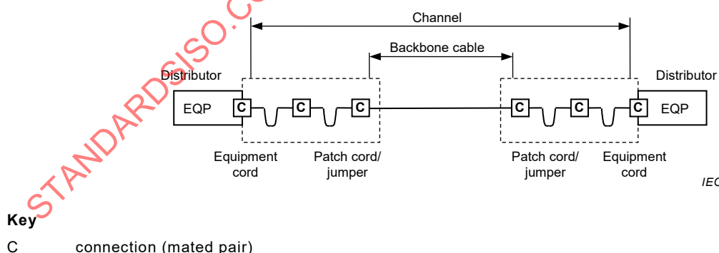
Figure 8 – Backbone cabling model
