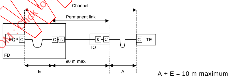
Figure 7c – Optical fibre cabling (with interconnect)
