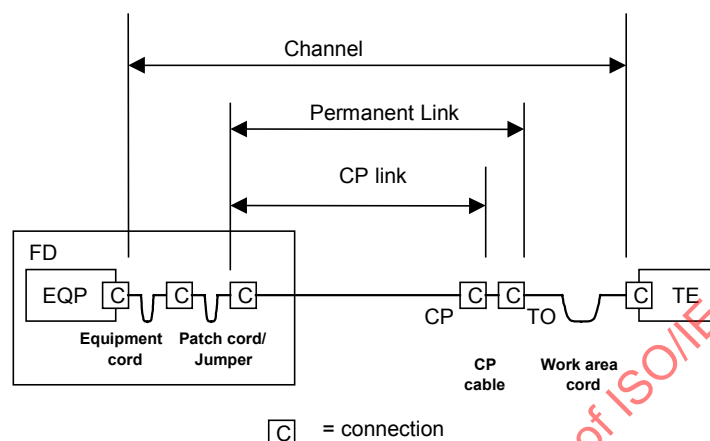
Figure 10 – Channel, permanent link and CP link of a balanced cabling
