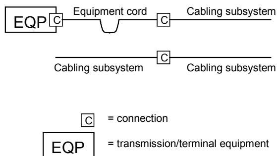
Figure 5 – Interconnect models
