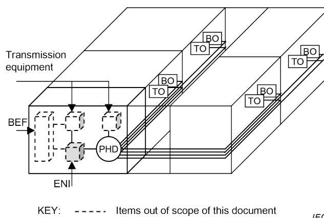
Figure 9 – Overview of a generic cabling for home
