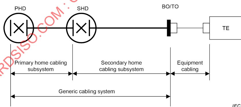
Figure 2 – Structure of the generic cabling system
