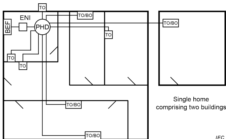
Figure 10 – Interconnection of home cabling subsystems
