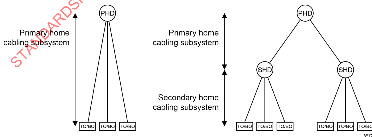
Figure 5 – Hierarchical structure of a generic cabling system in support of ICT and BCT applications
