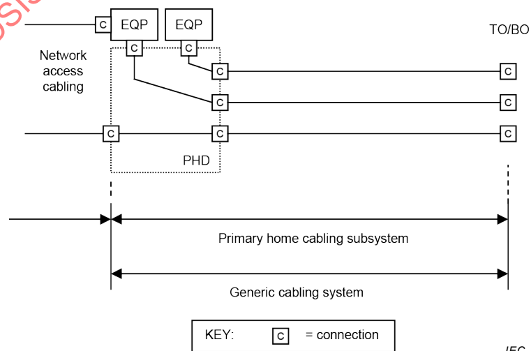
Figure 3 – Interconnect and cross-connect models
