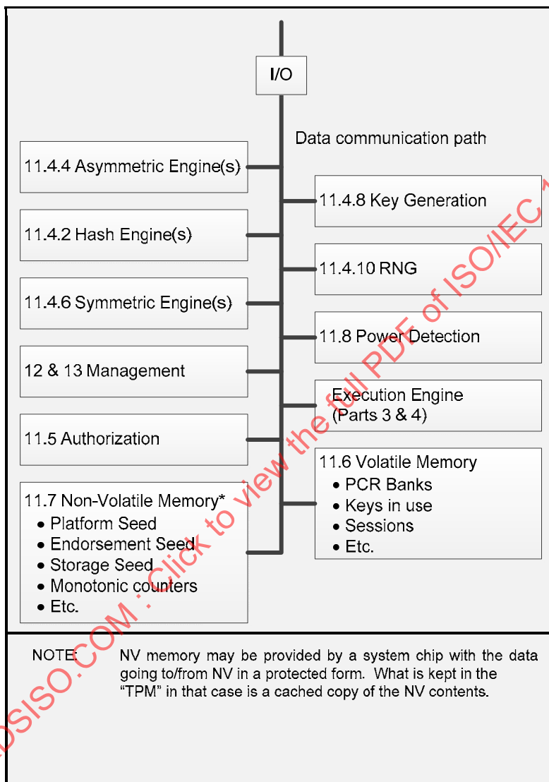
Figure 2 — Architectural Overview
