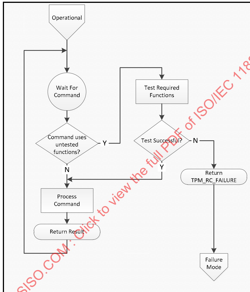
Figure 6 — On-Demand Self-Test
