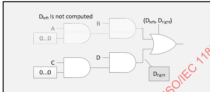
Figure 19 — Policy where only one OR Branch is Evaluated
