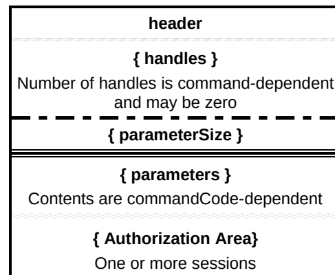
Figure 11 — Response Structure
