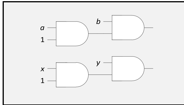
Figure 16 — Two Different Policy Expressions
