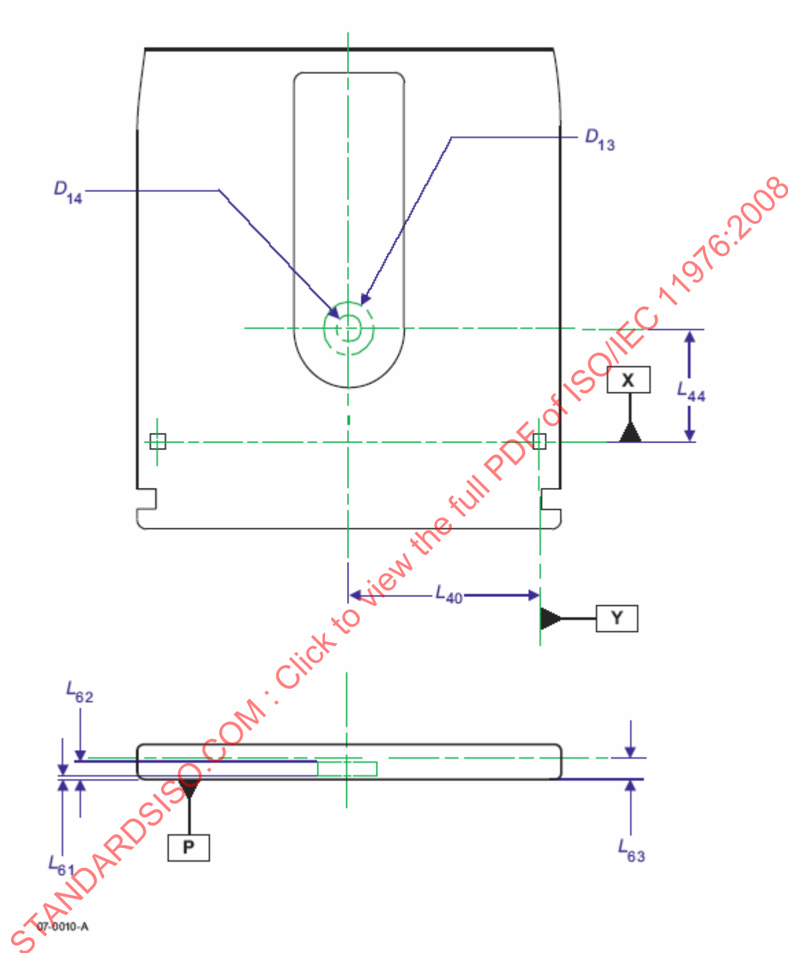
Figure 13 — Capture cylinder
