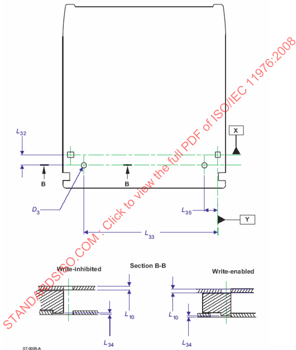
Figure 7 — Write-inhibit holes
