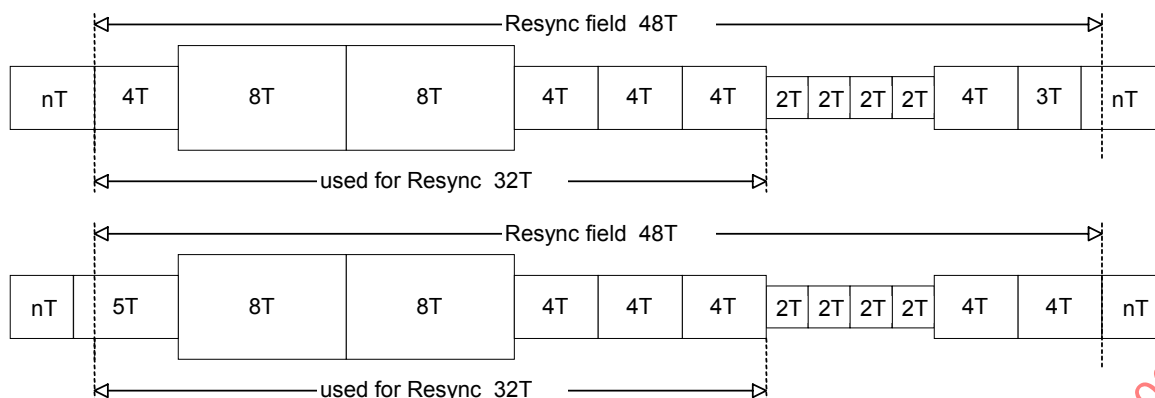
Figure 21 — Runlengths of the Resync field for different data bits
