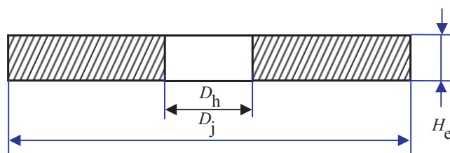
Figure F.2 — Calibration plate of the test device
