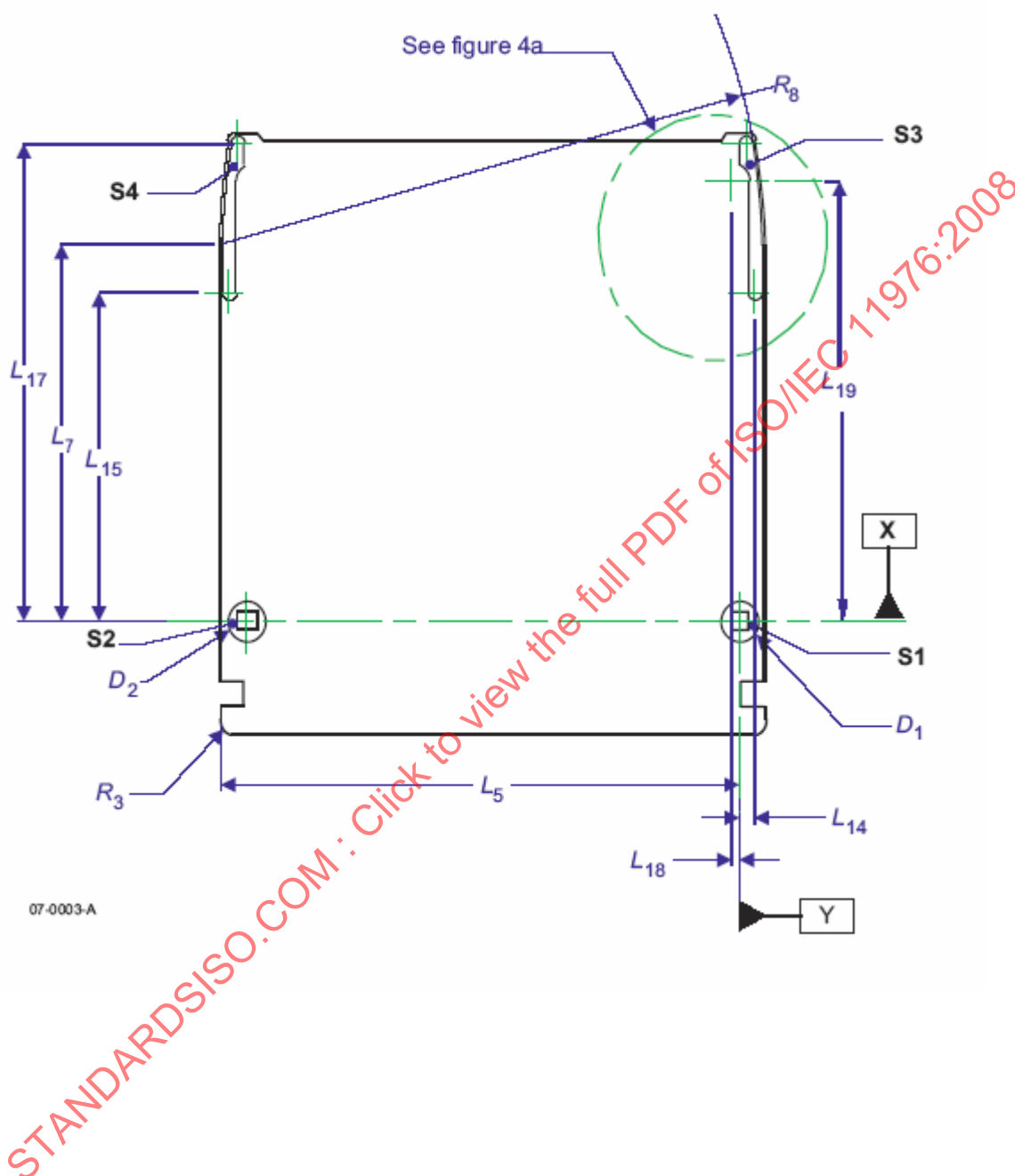
Figure 4 — Surfaces S1, S2, S3 and S4 of the Case Reference Plane P
