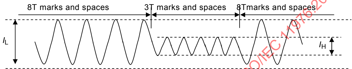
Figure 25 — Definition of I_L and I_H for resolution measurement
