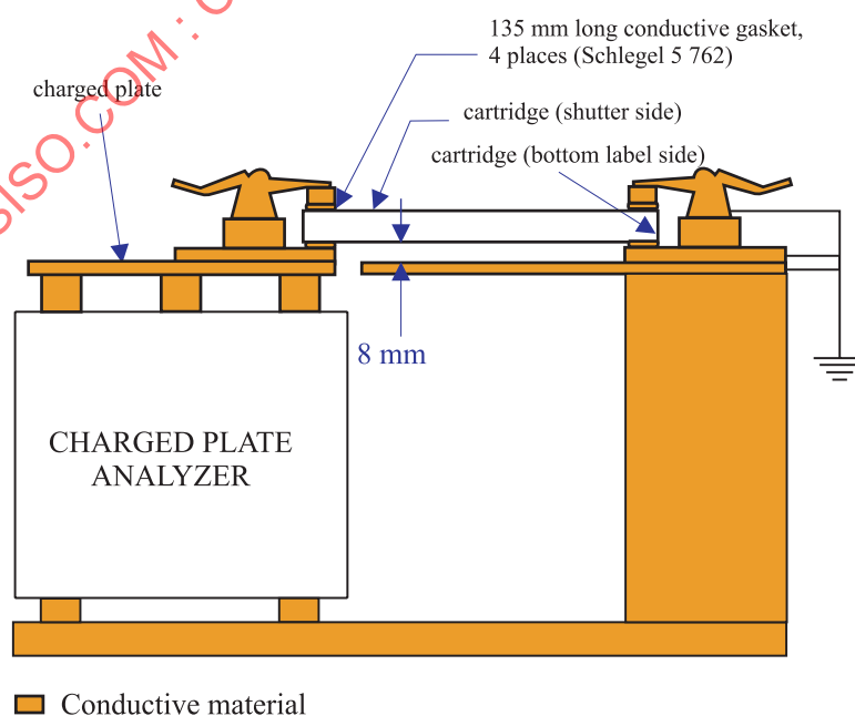
Figure E.1 — Cartridge electro-static discharge test fixture
