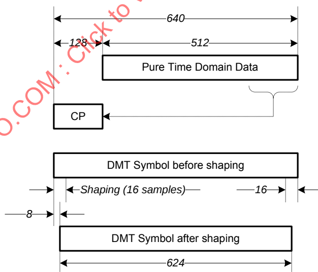
Fig. 16 - Cyclic Prefix and Shaping
