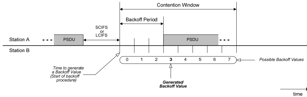
Fig. 24 - Example of Backoff Procedure
