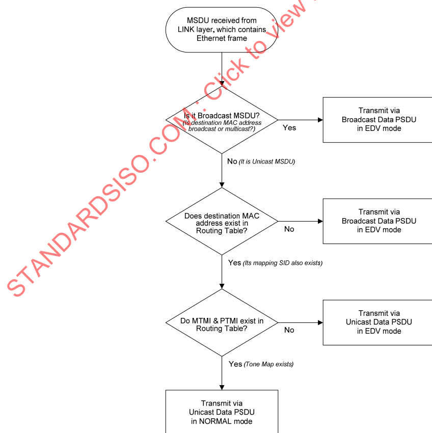
Fig. 39 - Flowchart for Settlement of Delimiter Form and Initial Transmission Mode
