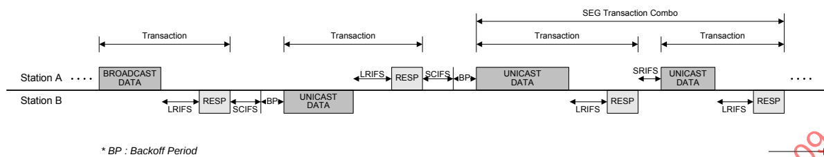
Fig. 25 - Example of Frame Transmission
