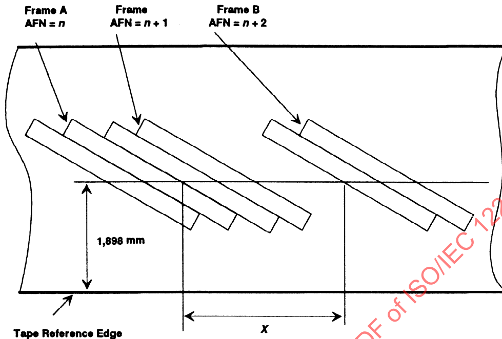
Figure 49 - Tolerance on seamless appending
