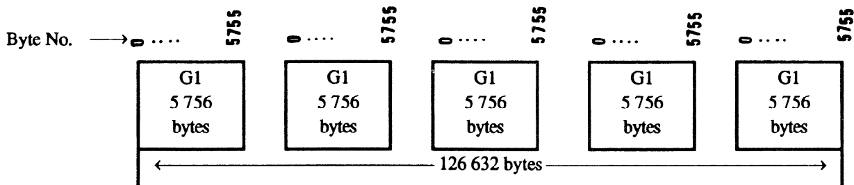
Figure 27 - G1 Sub-Groups
