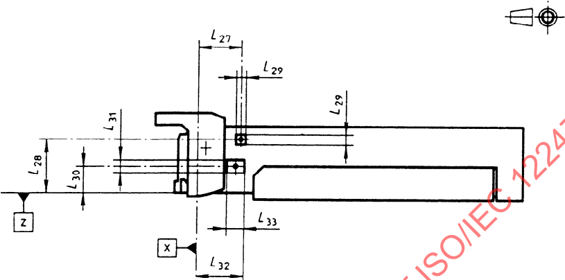
Figure 9 - Left side, lid open
