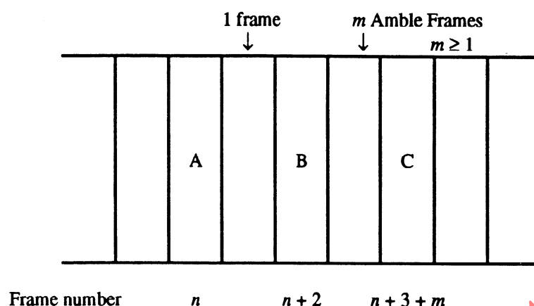
Figure 48 - Appending rules
