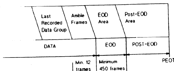
Figure 47 - Layout of a Single Data Space tape
