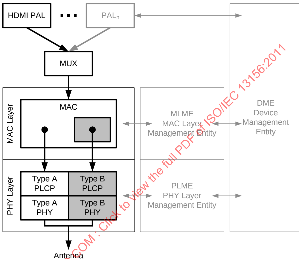
Figure 1 - Protocol structure
