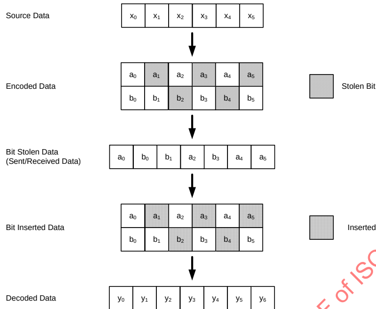
Figure 21 - An example of bit-stealing and bit-insertion for R=6/7 code
