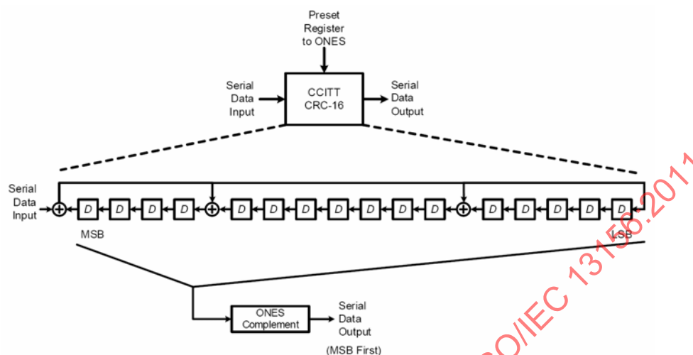
Figure 10 - CCITT CRC-16 block diagram
