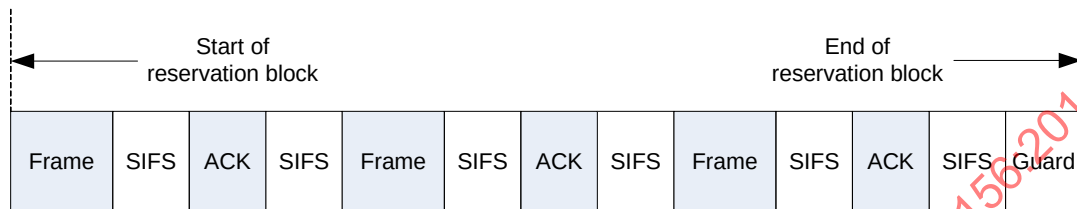
Figure 168 - SIFS and guard time in a DRP reservation block - Imm-ACK
