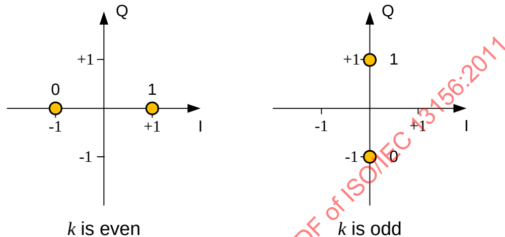
Figure 34 - BPSK constellation bit encoding
