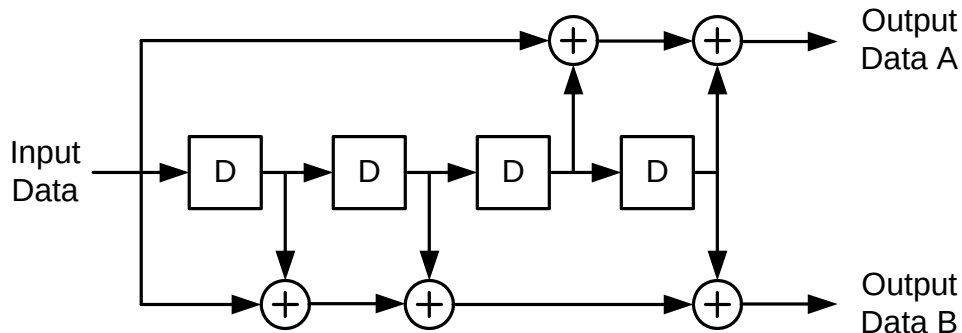
Figure 16 - Convolutional encoder: rate R=1/2 , constraint length K=5
