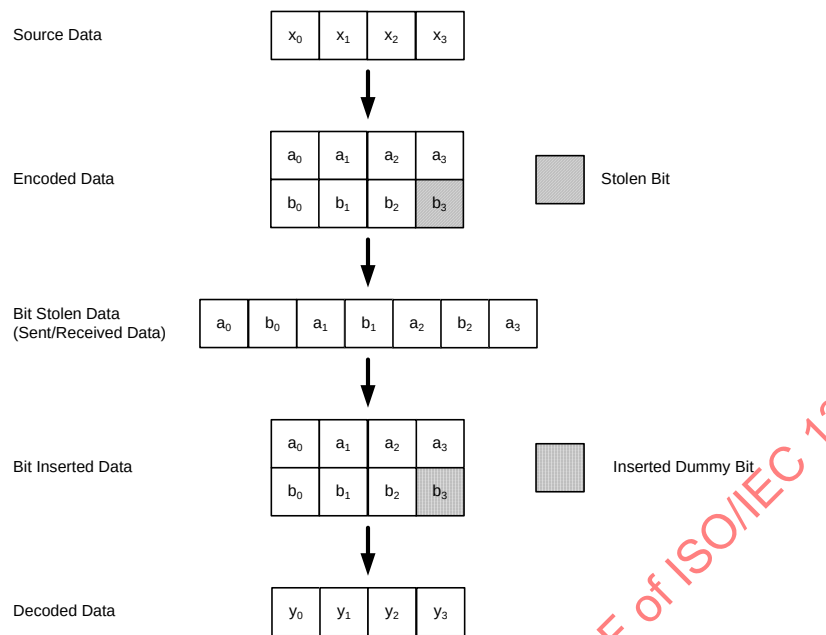
Figure 17 - An example of bit stealing and bit insertion for R=4/7 code
