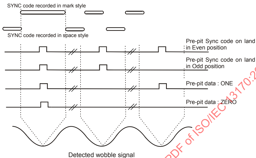
Figure 49 — Relationship of signals recorded in groove and land
