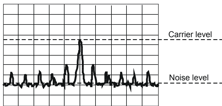
Figure 18 — Measurement of the wobble CNR
