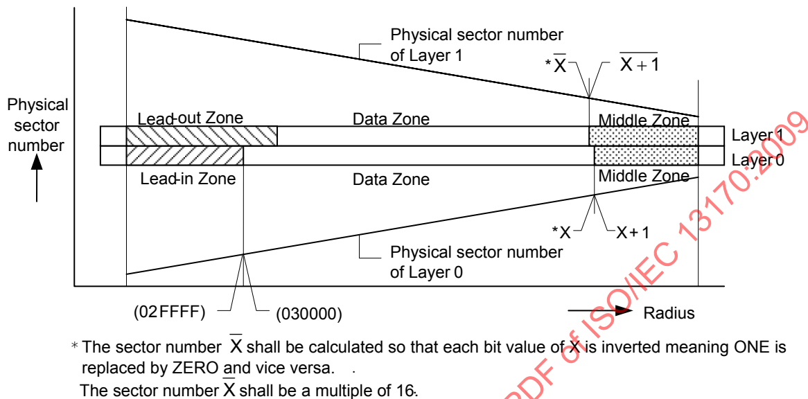
Figure 40 — Physical Sector numbering
