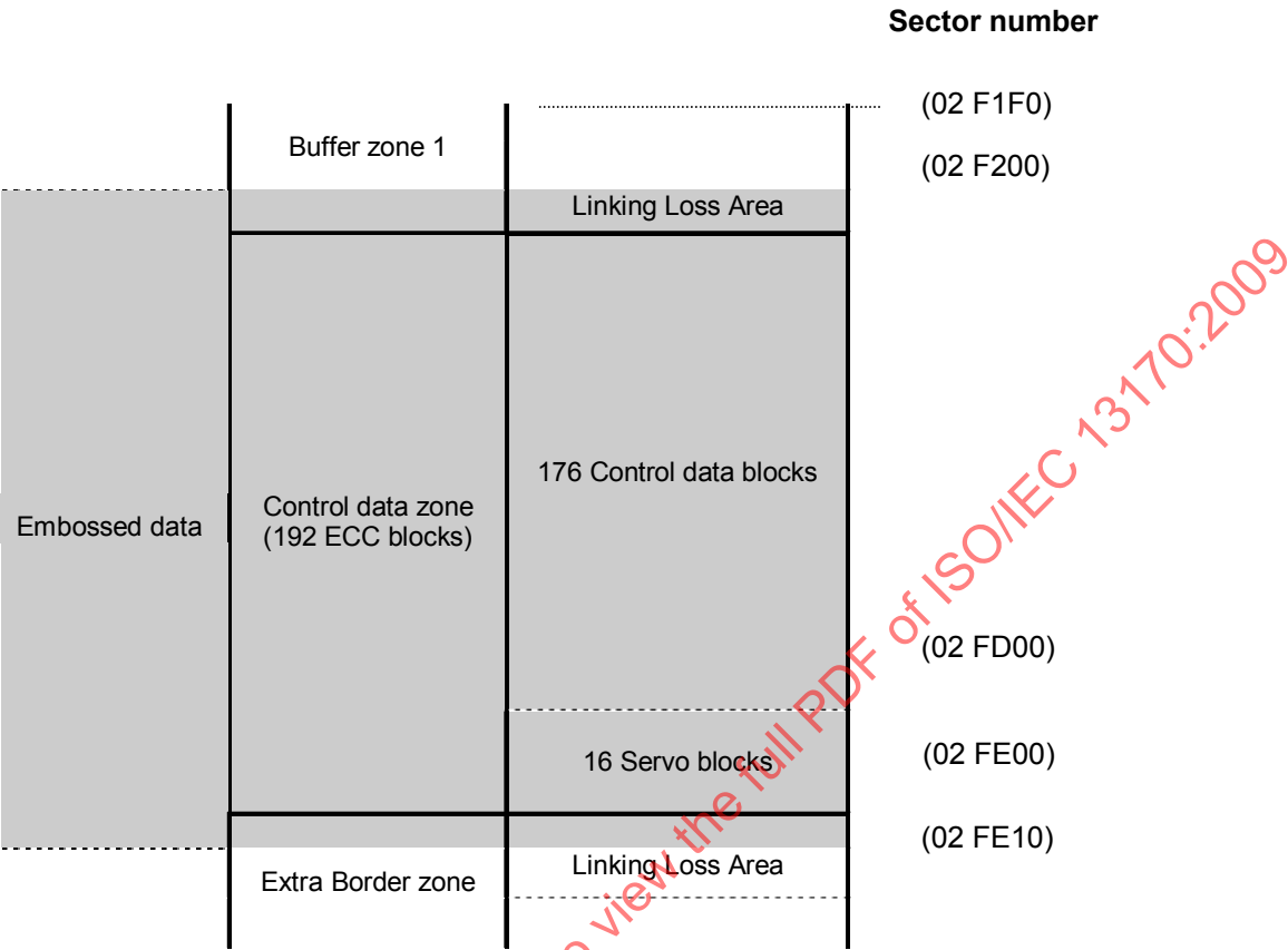
Figure 43 — Structure of a Control data Zone
