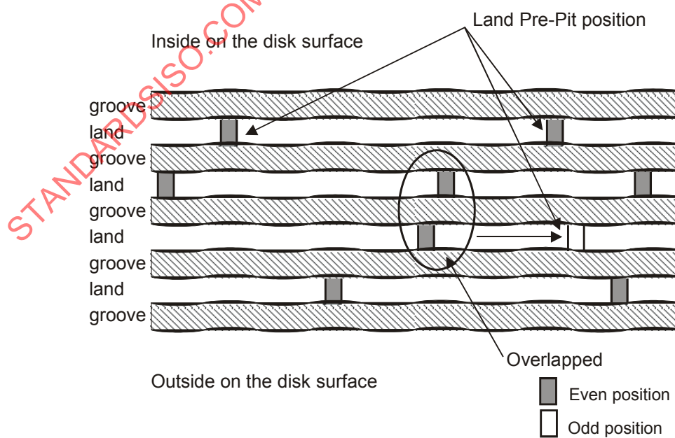
Figure 50 — Layout of land Pre-pit positioning
