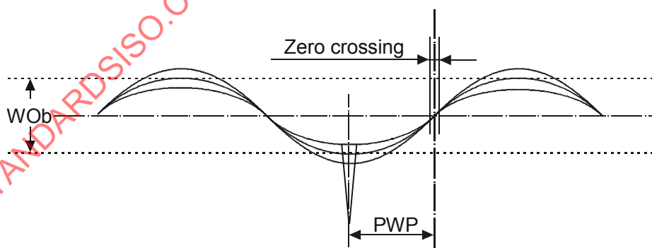
Figure 26 — Relation in phase between wobble and Land Pre-Pit
