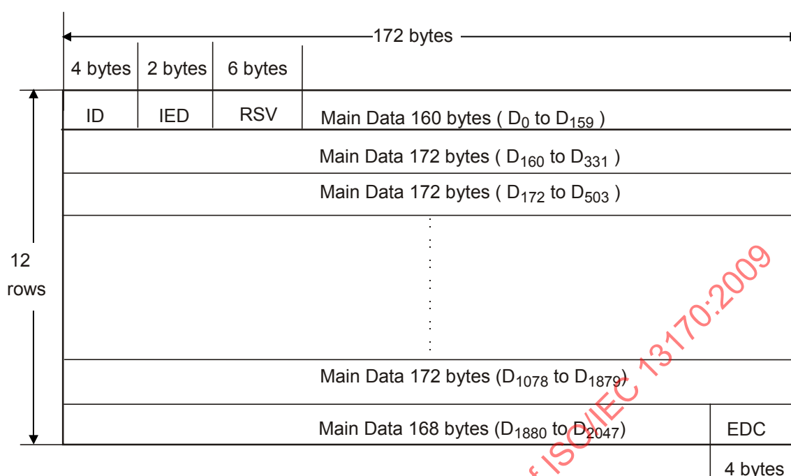
Figure 28 — Data Frame
