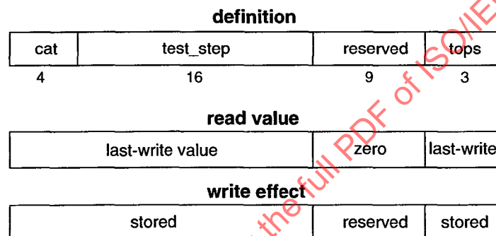
Figure 37—TEST_START format
