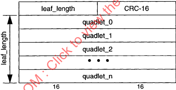
Figure 62—Leaf format
