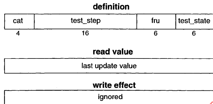
Figure 39—TEST_STATUS format
