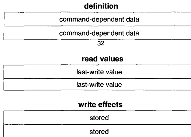
Figure 35—ARGUMENT formats
