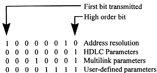
Figure 22 — General purpose XID data link layer subfield identifier encodings
