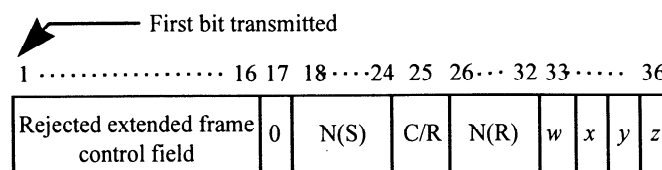
Figure 18b — Information field format for FRMR response in modulo 128 operation
