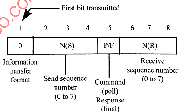
Figure 3a — Information transfer format of control field bits for modulo 8 numbering
