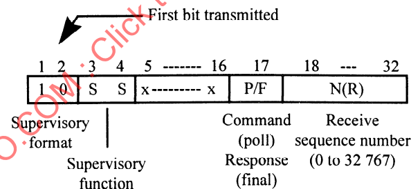
Figure 4c — Supervisory format of control field bits for modulo 32 768 numbering
