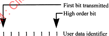
Figure 23 — User data subfield encoding
