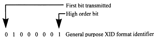
Figure 21 — General purpose XID format identifier subfield encoding
