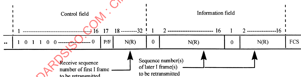
Figure 5c — Control field and information field encoding in SREJ frame for modulo 32 768 numbering
