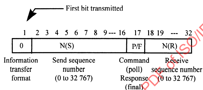
Figure 3c — Information transfer format of control field bits for modulo 32 768 numbering
