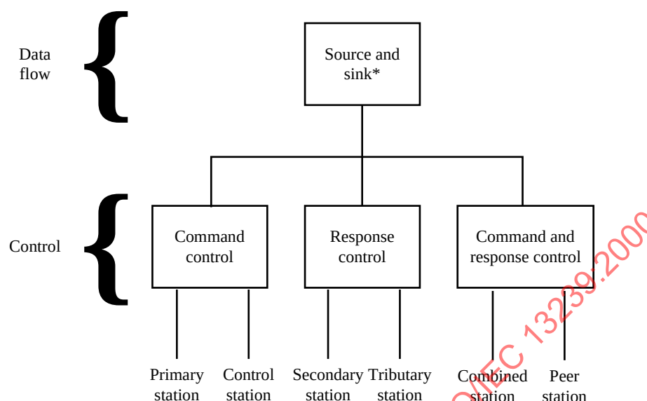
Figure 19 — HDLC stations — Building blocks
