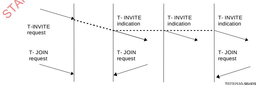
Figure 8 – Sequence of primitives in a TC Invitation
