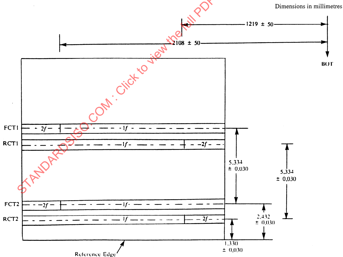
Figure 22 - Calibration Tracks Area
