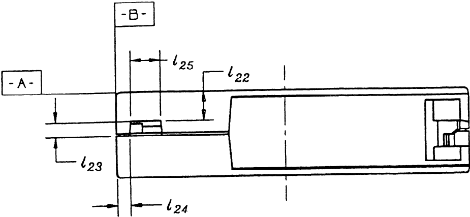
Figure 10 - Back side
