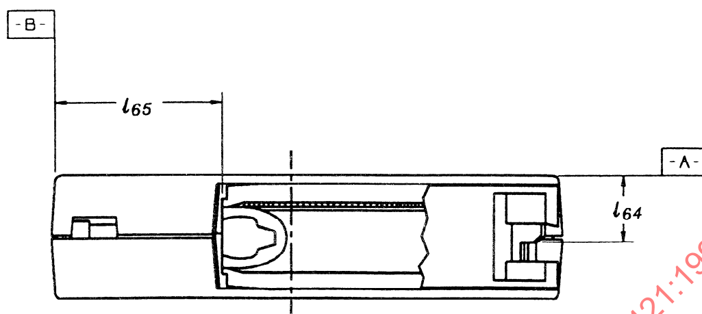
Figure 18 - Back side, position of the door lock
