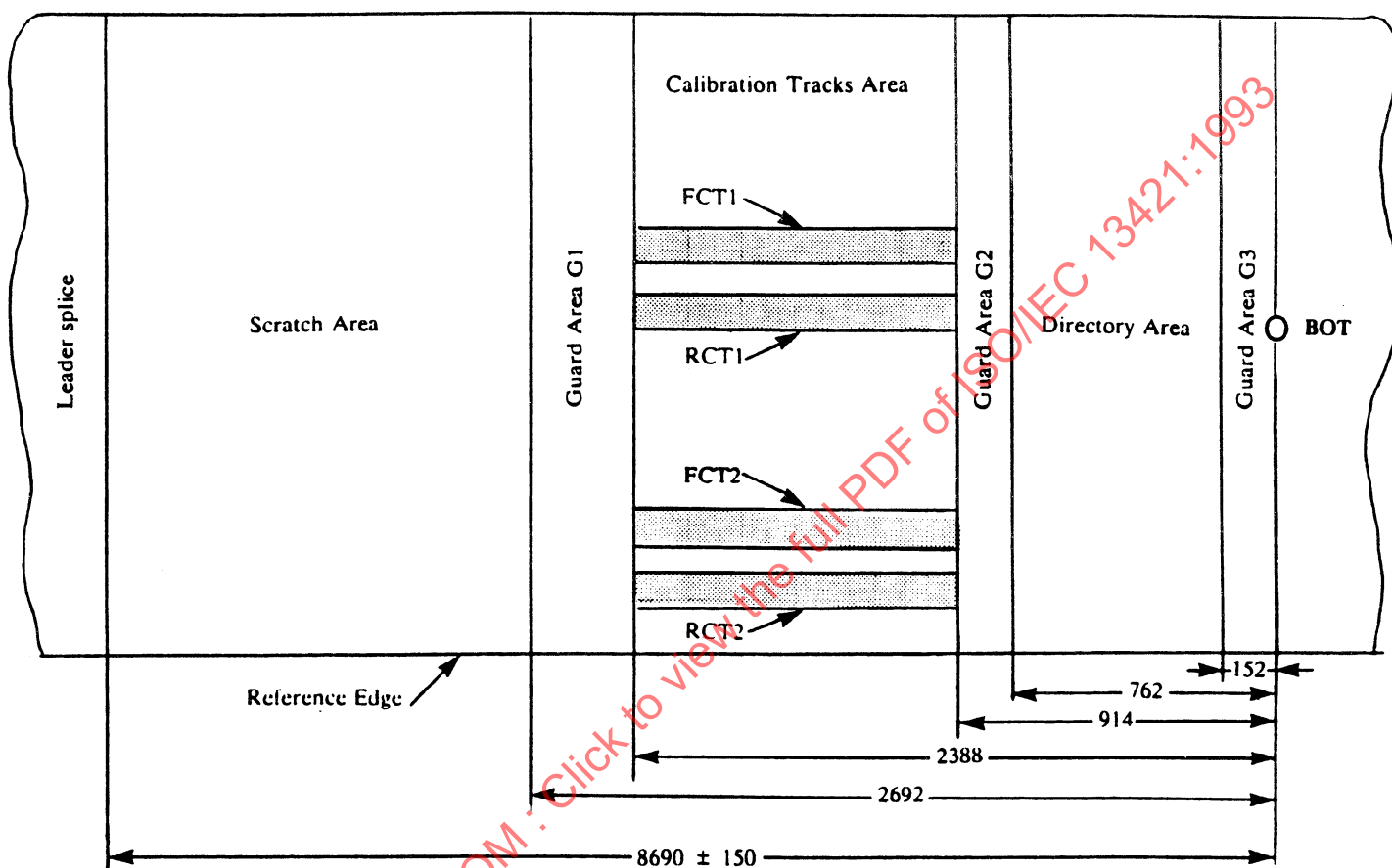
Figure 21 - Calibration and Directory Area
