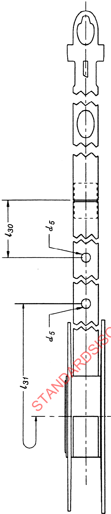
Figure 14 - Leader/tape connection
