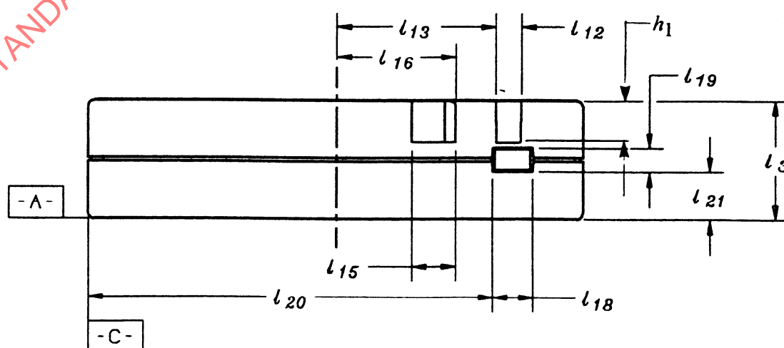
Figure 9 - Right side
