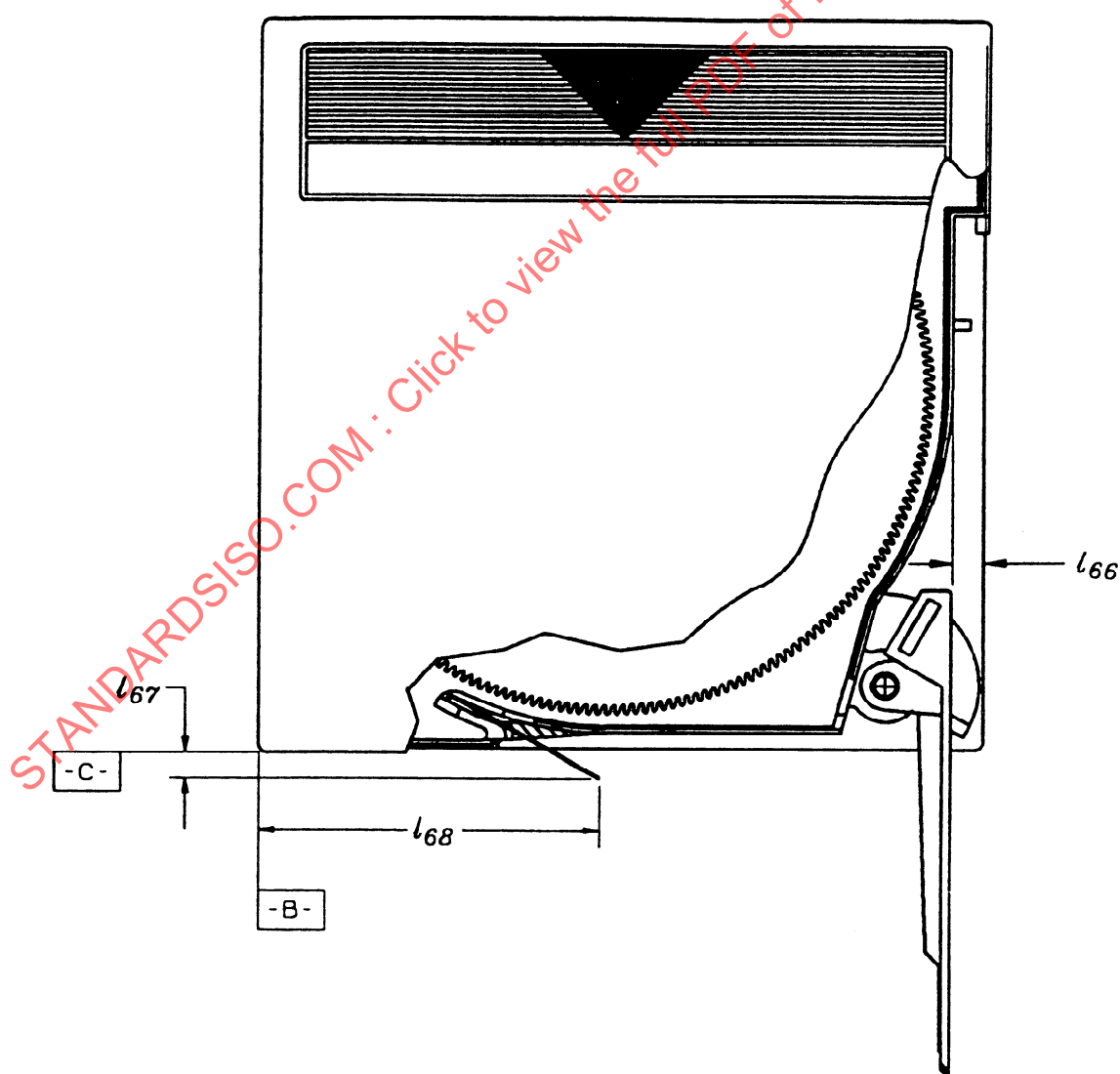
Figure 19 - Position of the leader tip
