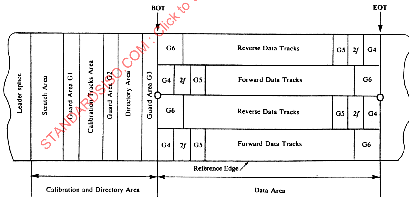
Figure 20 - Tape layout
