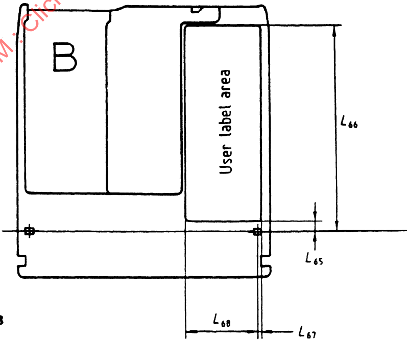
Figure 14.c - User label area on Side B
