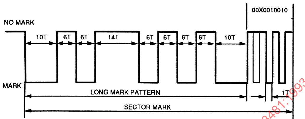
Figure 21 - Sector Mark pattern
