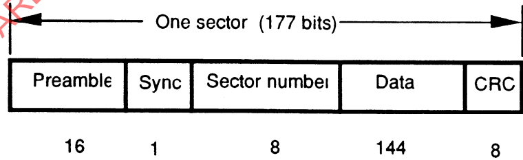
Figure 18 - Sector format in the PEP Zone
