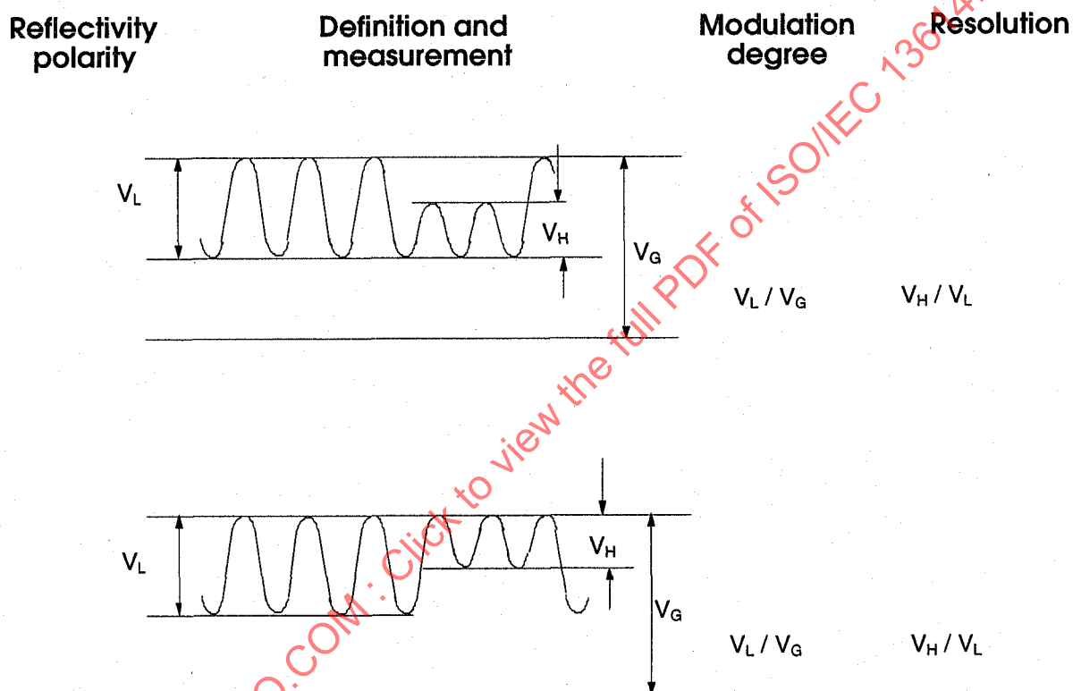
Figure 25 - Reflectivity characteristics of user-written data
