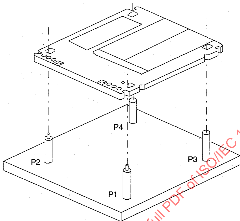
Figure B.1 - Compliance gauge
