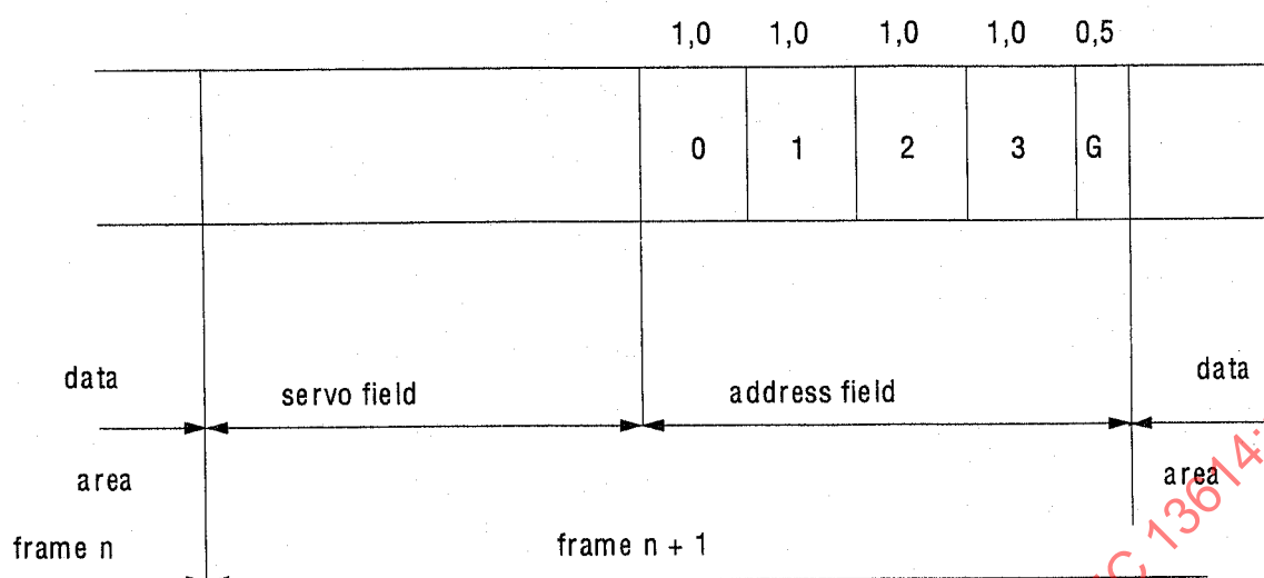
Figure 16a - Address field of an even-numbered frame
