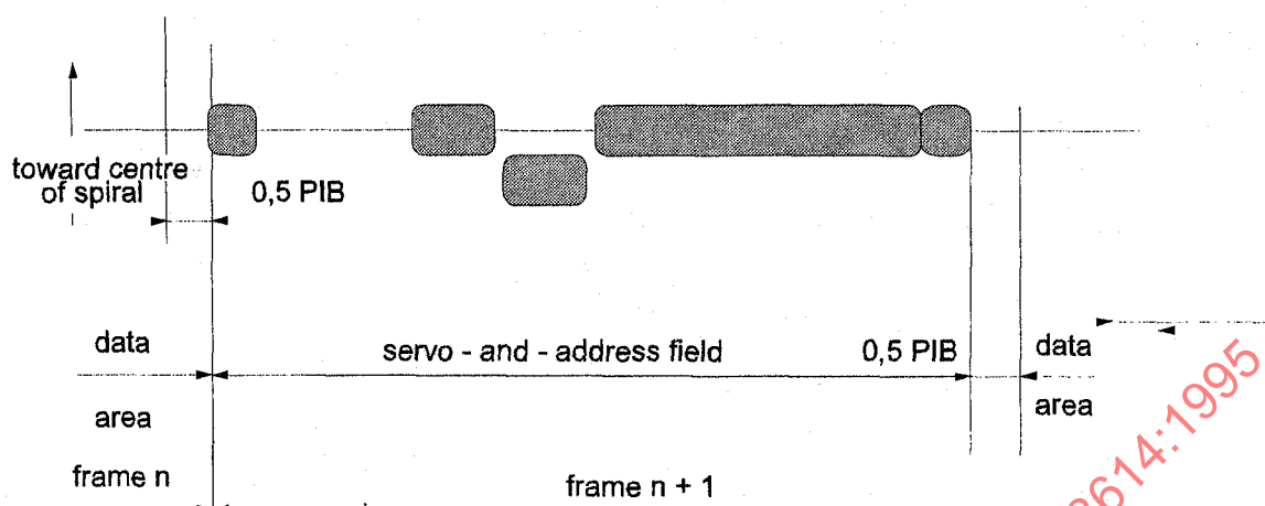
Figure 20b - Disk without groove. Even track. Odd frame
