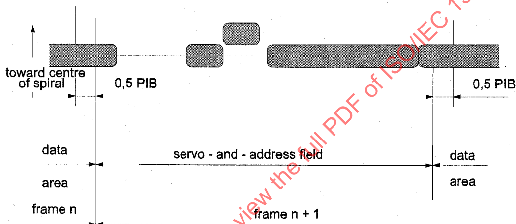
Figure 20a - Disk with long part of a groove. Even track. Even frame
