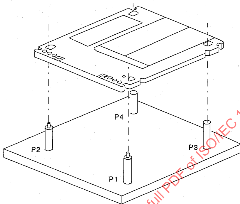
Figure A.1 - Distortion gauge
