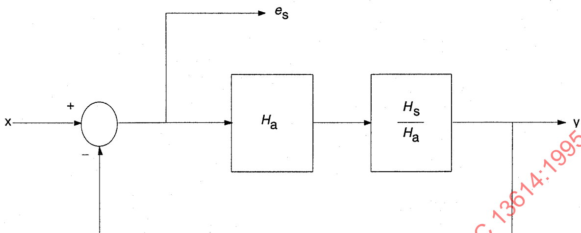
Figure C.3 - Implementation of a reference servo by changing the transfer function of the actual servo
