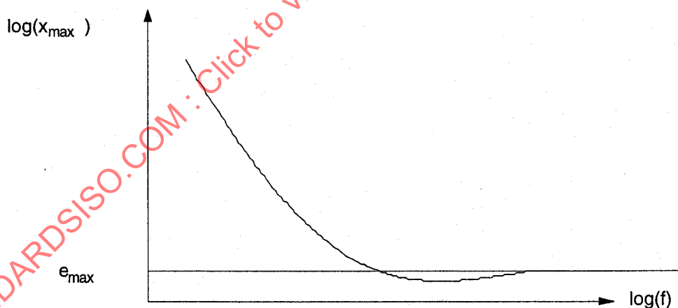
Figure C.1 - Maximum allowed amplitude of a single, sinusoidal track deviation
