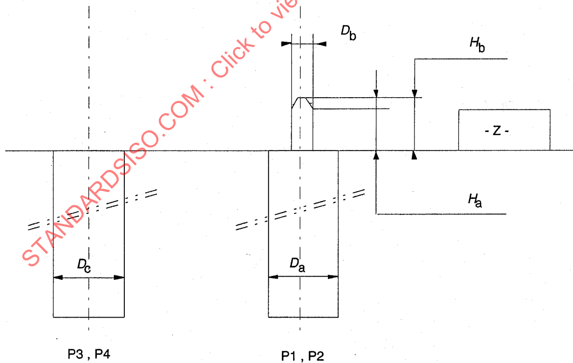
Figure B.2 - Details of posts
