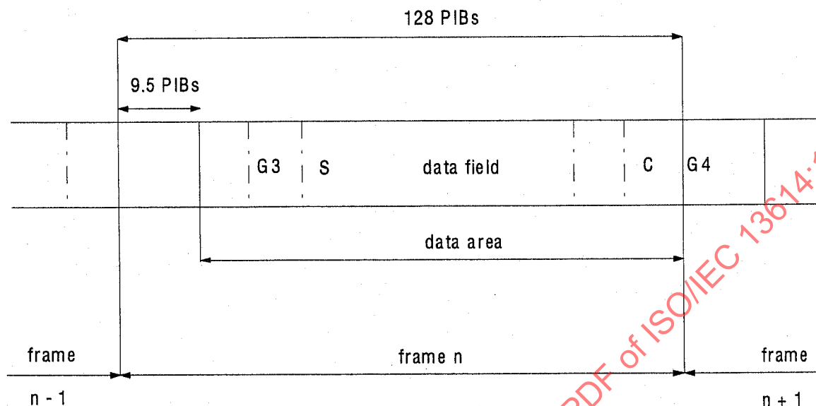
Figure 19 - Data area
