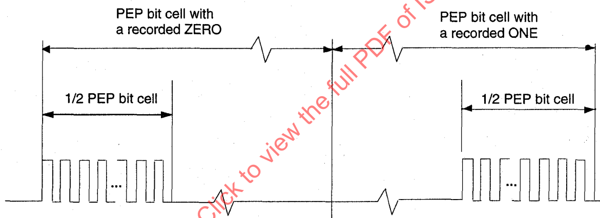
Figure F.1 - Example of phase-encoded modulation in the PEP Control Zone
