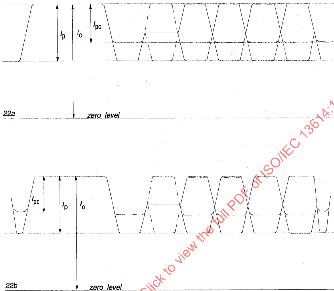
Figure 22 - Signals from the servo-and-address field
