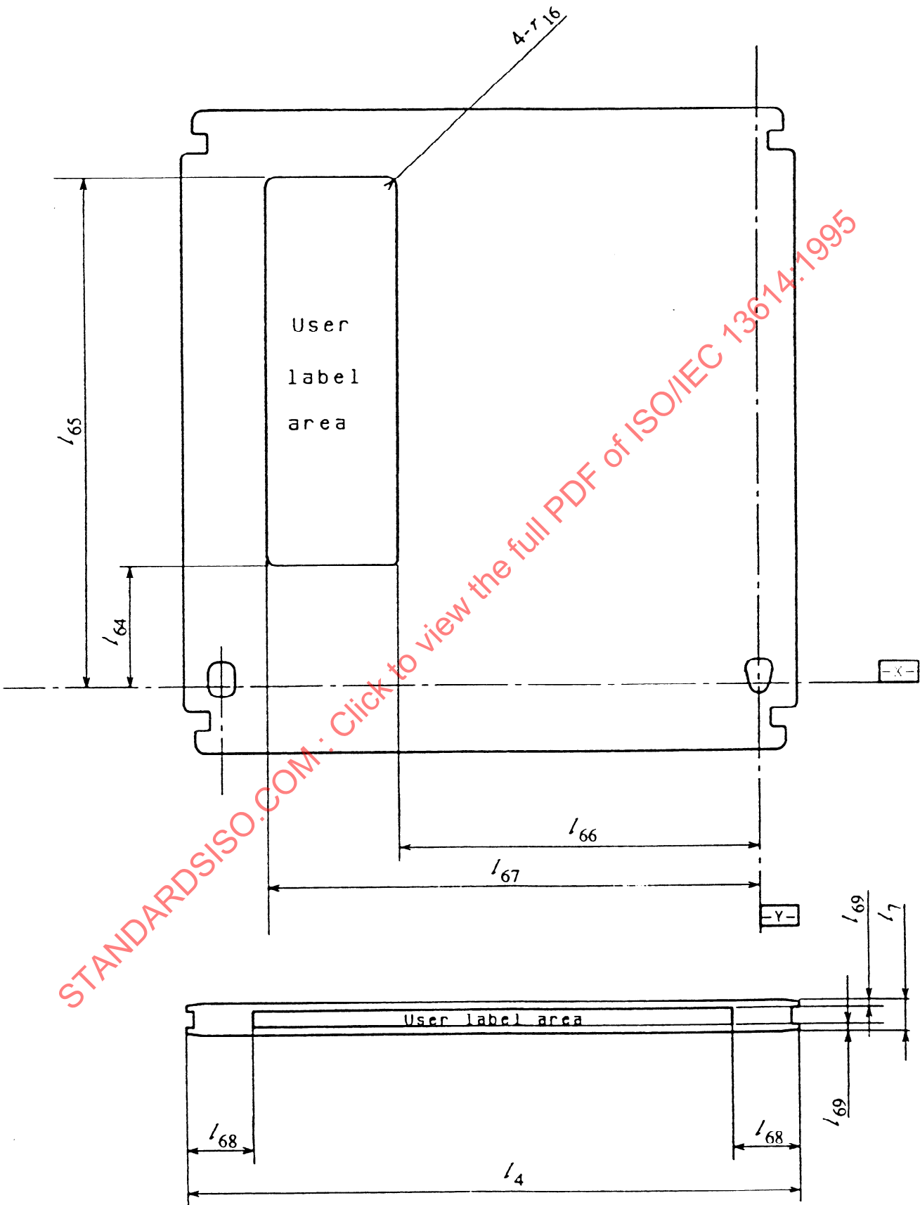
Figure 12 - Label area
