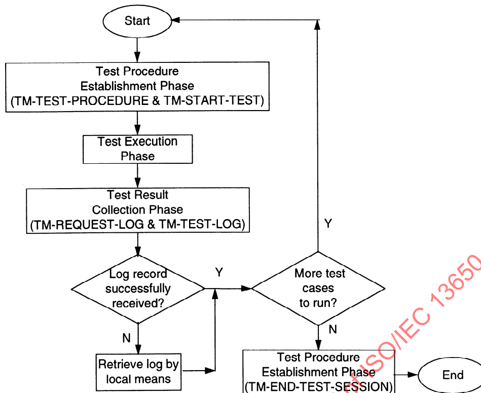
Figure 1 — Control flow for a test session
