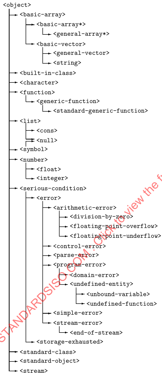
Figure 1. Class Inheritance
