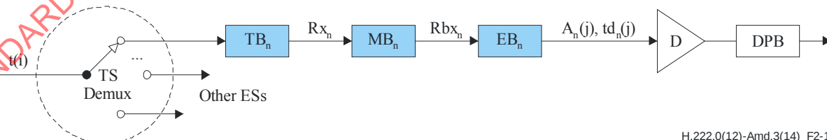
Figure 2-18 – T-STD model extensions for single layer HEVC
