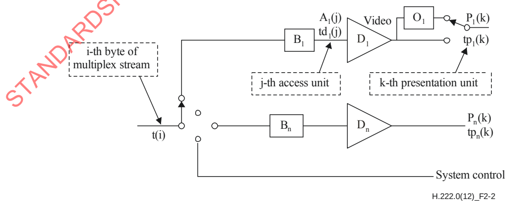
Figure 2-2 – Program stream system target decoder notation
