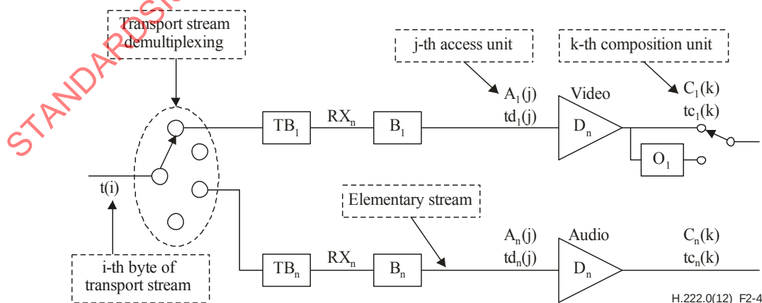
Figure 2-4 – T-STD model extensions for individual ISO/IEC 14496 elementary streams
