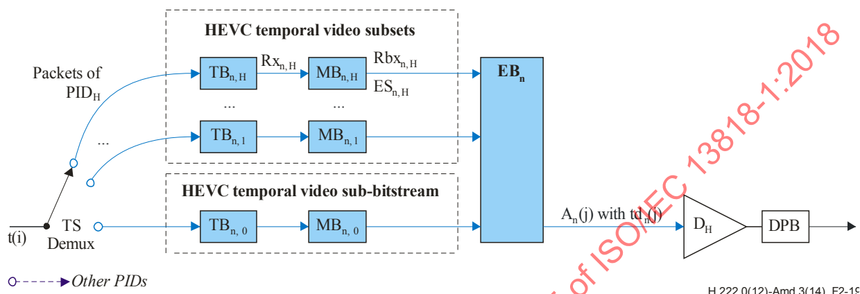
Figure 2-19 – T-STD model extensions for layered transport of HEVC temporal video subsets
