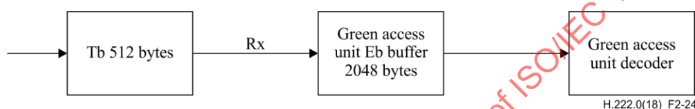
Figure 2-24 – T-STD model extension for green access units
