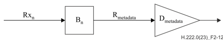
Figure 2-12 – Metadata decoding in the STD
