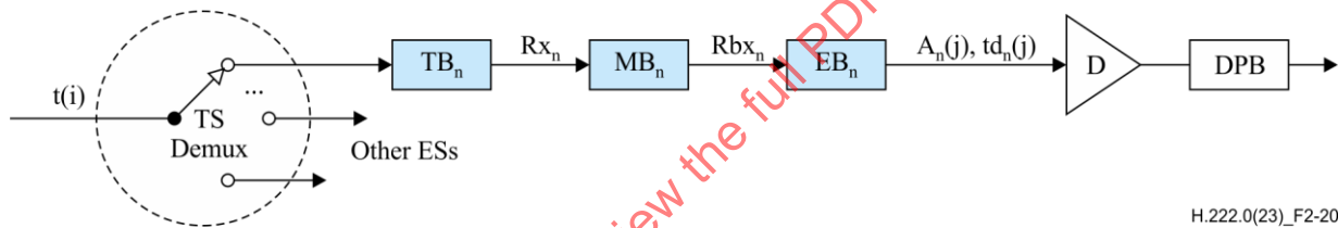
Figure 2-20 – T-STD model extensions for single layer HEVC
