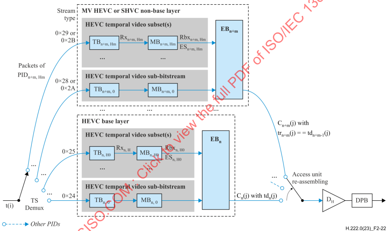
Figure 2-22 – T-STD model extensions for bitstream-partition-specific CPB operation
