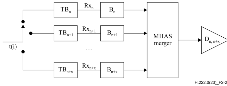
Figure 2-27 – Transport stream system target decoder for multiple audio elementary streams
