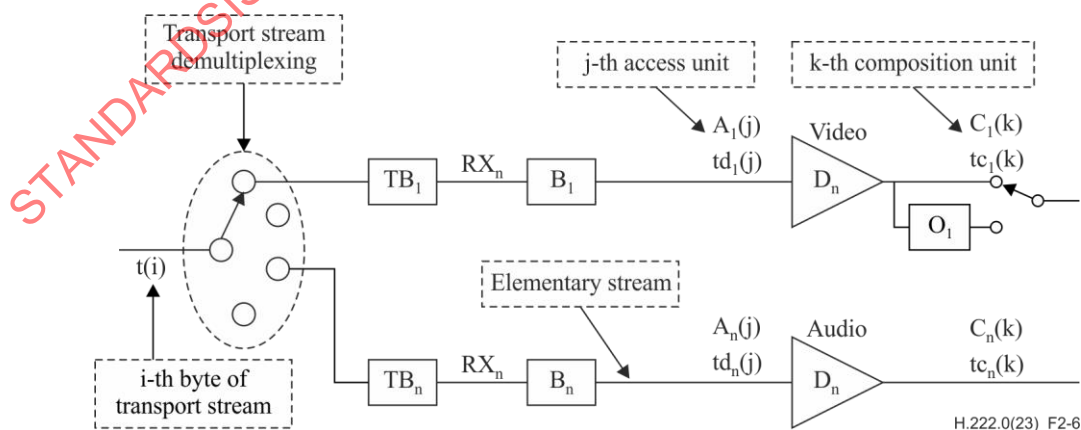
Figure 2-6 – T-STD model extensions for individual ISO/IEC 14496 elementary streams
