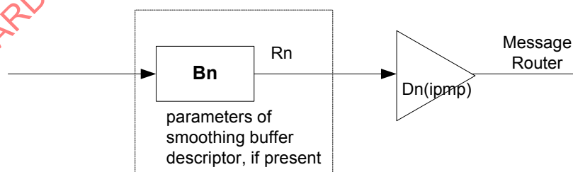
Figure 4 — IPMP Stream Decoder Model in Program Stream
