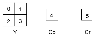
Figure 6-10 – 4:2:0 Macroblock structure
