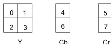
Figure 6-11 – 4:2:2 Macroblock structure
