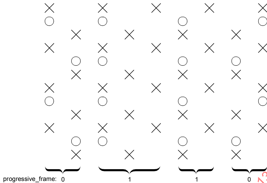
Figure 7-21 – progressive_sequence == 0 with 4:2:0 chrominance
