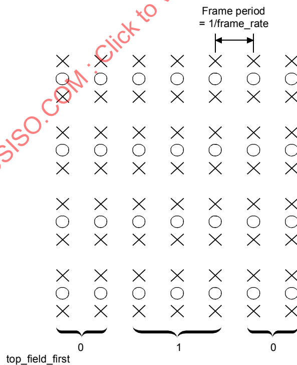
Figure 7-19 – progressive_sequence == '1'; repeat_first_field == '1'
