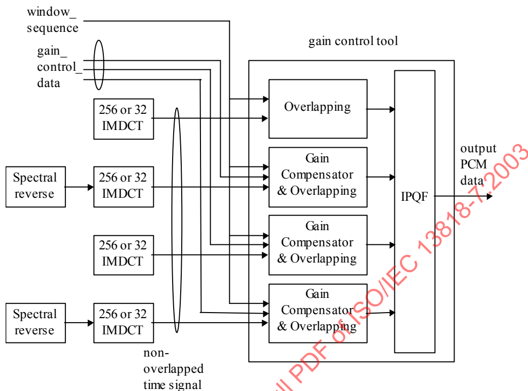
Figure 9 — Block diagram of gain control tool
