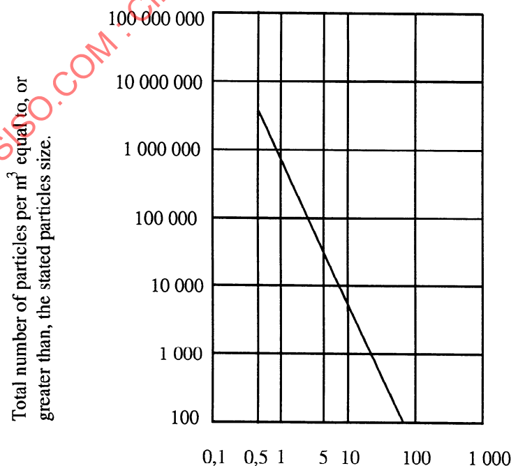
Figure A.1 - Particle size distribution curve
