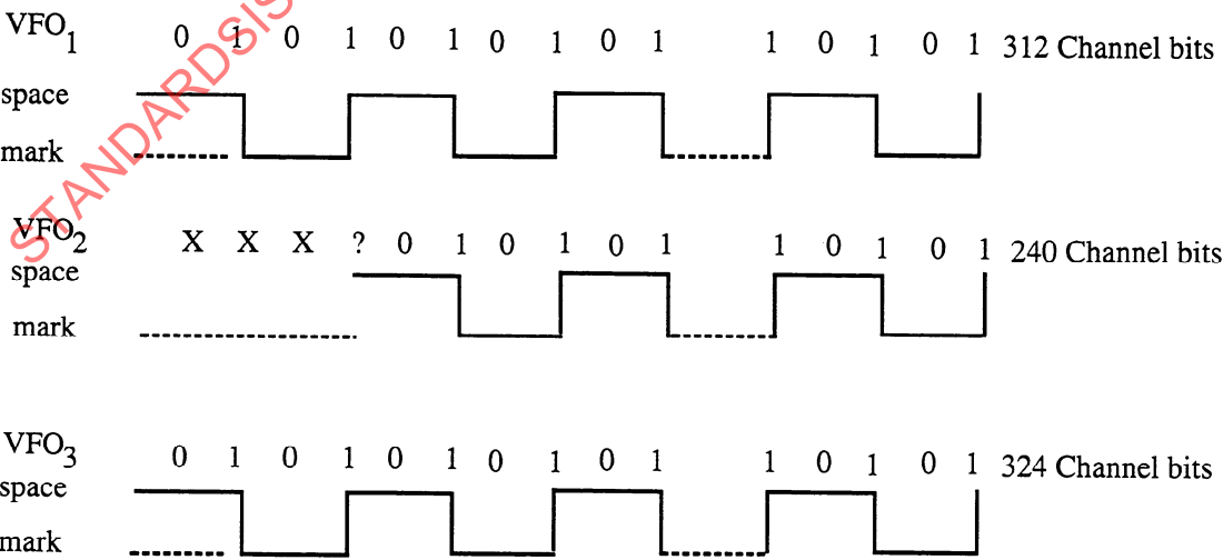
Figure 18 - VFO Field Patterns
