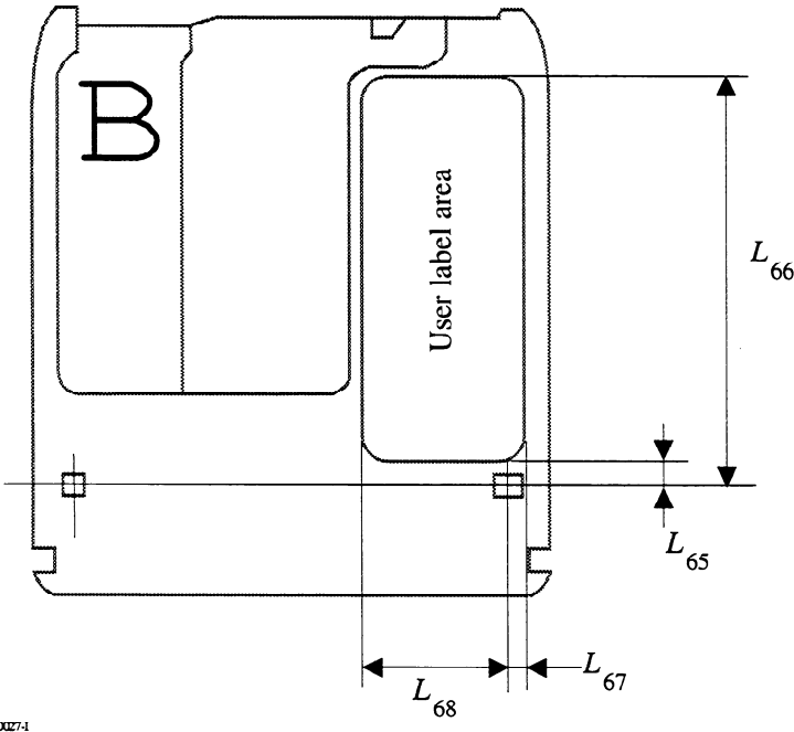
Figure 14 - User label area
