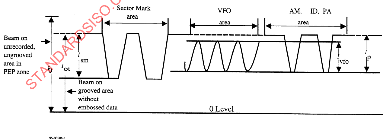
Figure 24B - Signals from Headers in Channel 1
