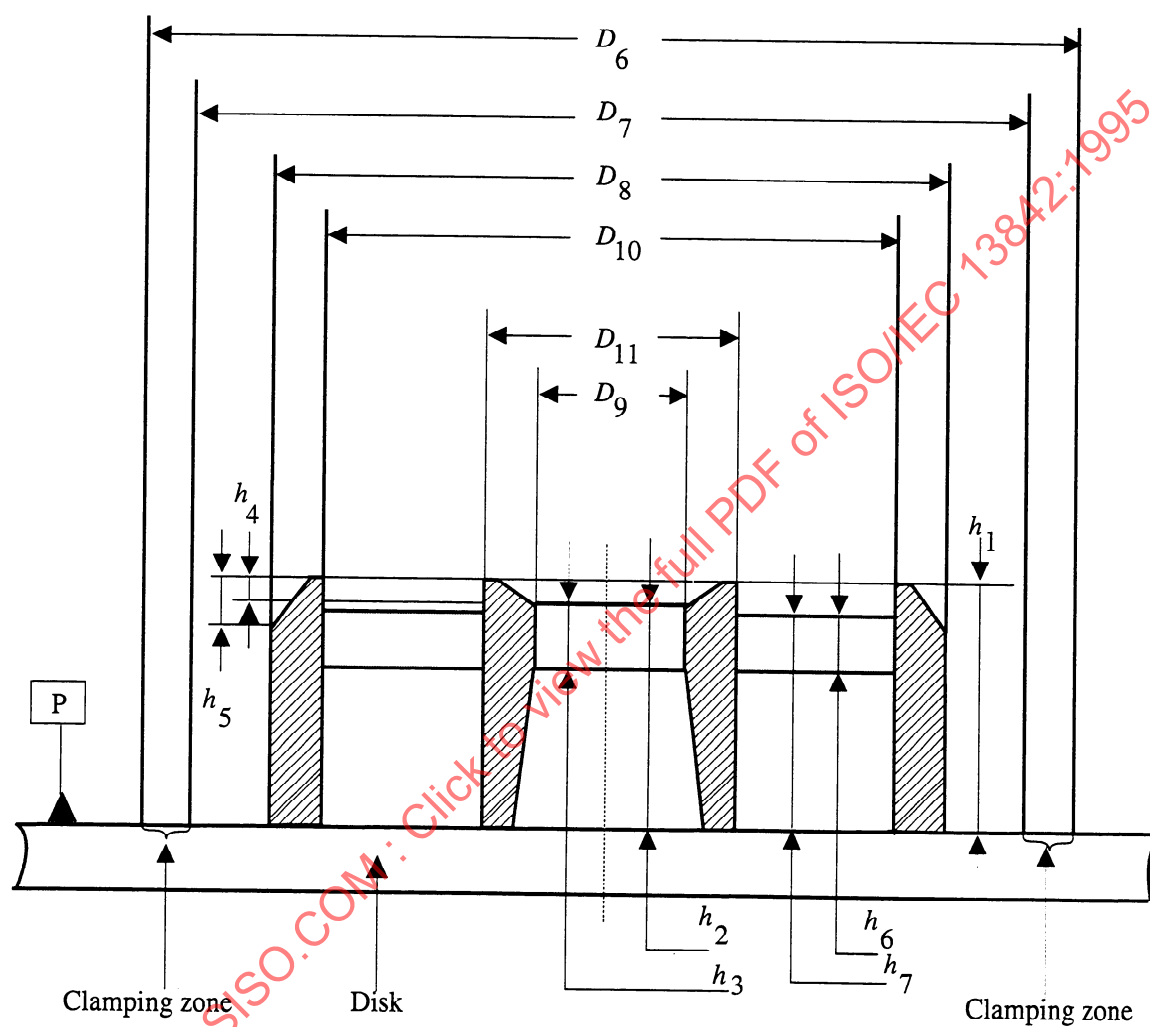
Figure 2 - Hub dimensions
