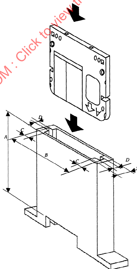
Figure B.1 - Distortion gauge
