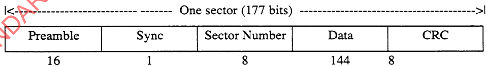
Figure 23 - Sector format in the PEP Zone
