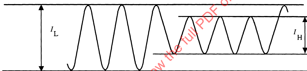
Figure 26 - Definition of I_L and I_H
