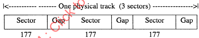
Figure 22 - Track format in the PEP Zone
