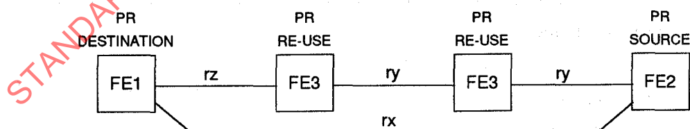
Figure 8 - Functional model for enhanced operation of ANF-PR
