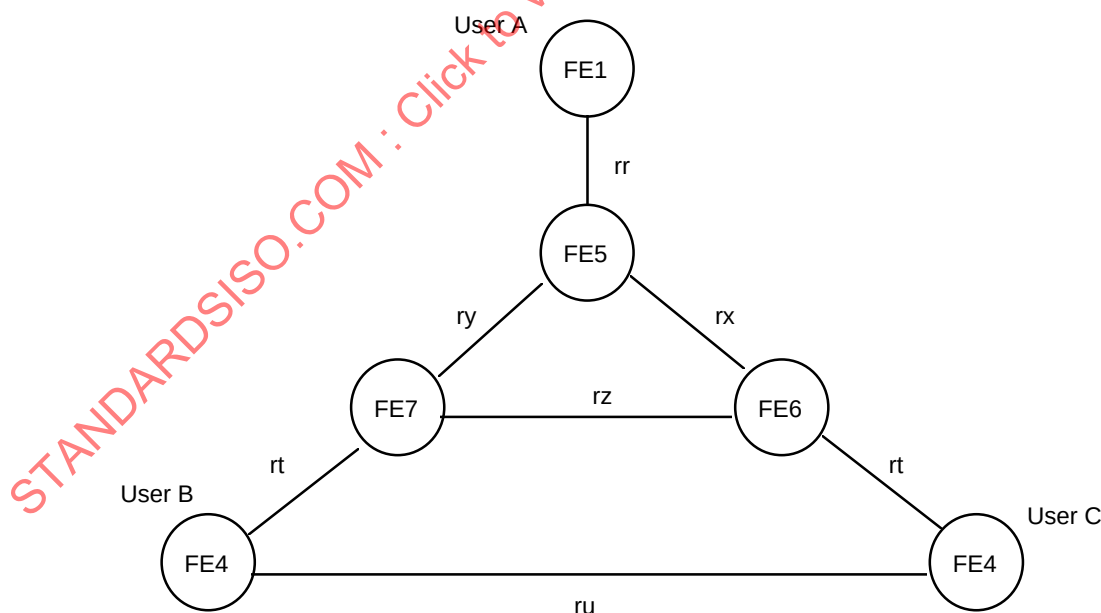
Figure 10 - Functional model of SS-CT
