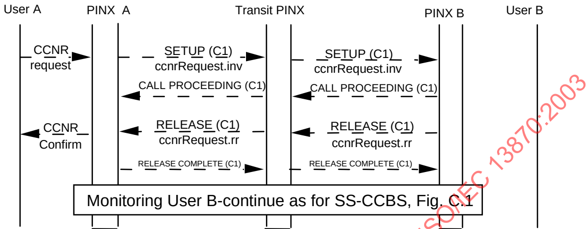
Figure C.3 - Example message flow for successful CCNR
