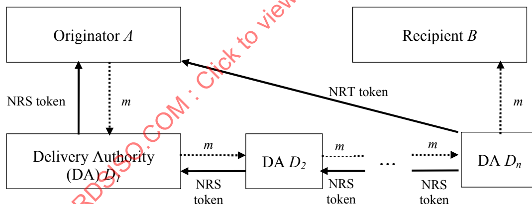
Figure 2 – Use of non-repudiation tokens with Delivery Authorities
