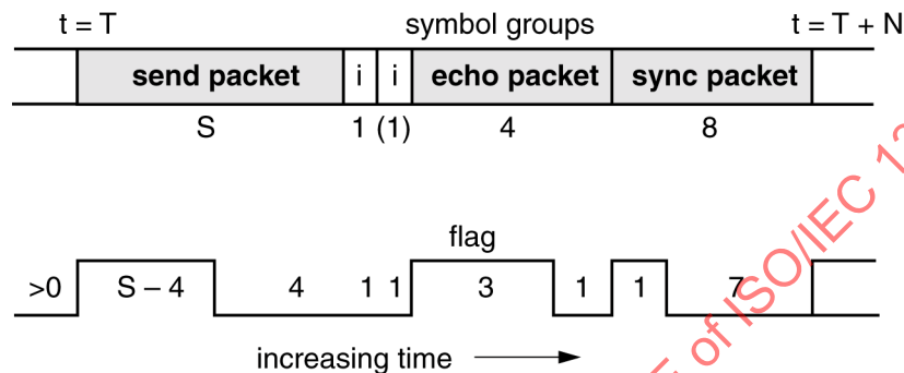
Figure 108 – Flag framing convention
