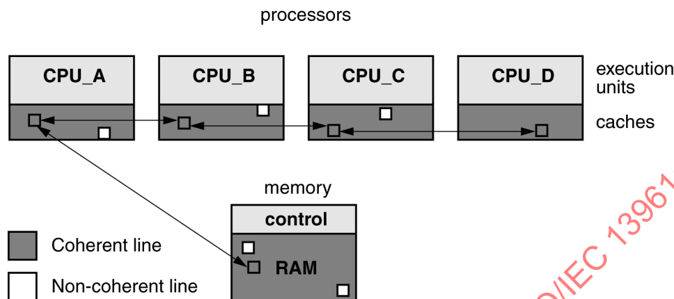
Figure 129 – Distributed sharing-list directory
