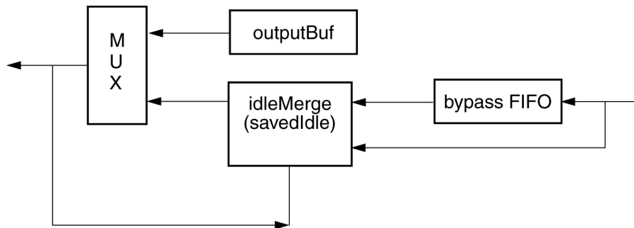
Figure 71 – Pass-transmission model (fair-only node)
