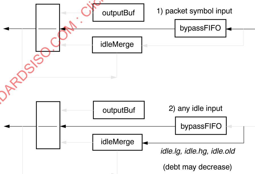
Figure 79 – Low/high-transmission debt repayment
