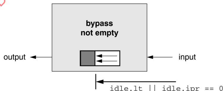
Figure 69 – Idle consumption, fair-only node
