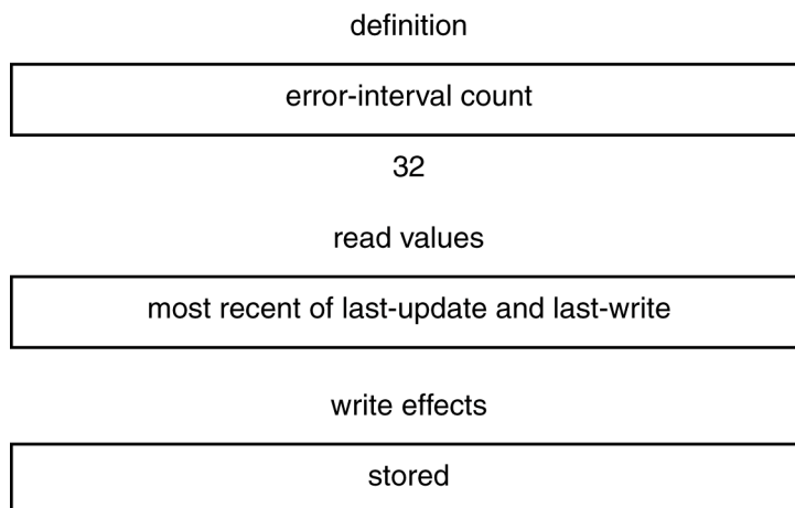
Figure 117 – ERROR_COUNT register (offset 384)
