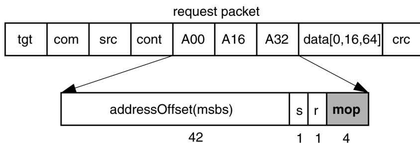
Figure 170 – Basic mread/mwrite request
