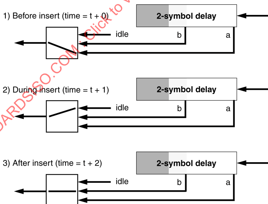
Figure 62 – Idle-symbol insertion
