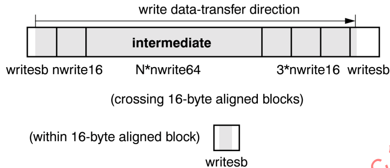
Figure 57 – Expected DMA write transfers
