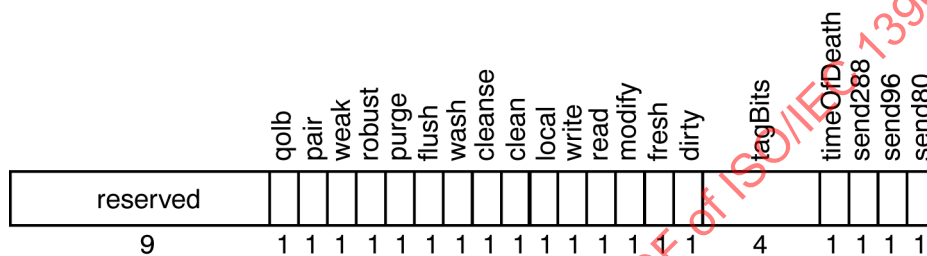
Figure 125 – ROM format, CacheOptions
