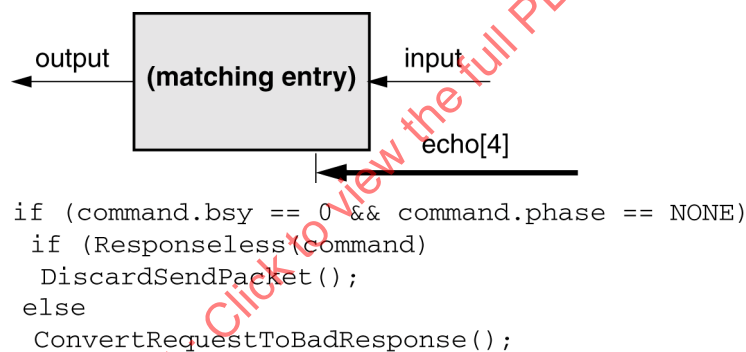
Figure 93 – Producer's address-error processing
