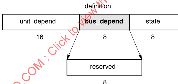
Figure 113 – STATE_CLEAR fields
