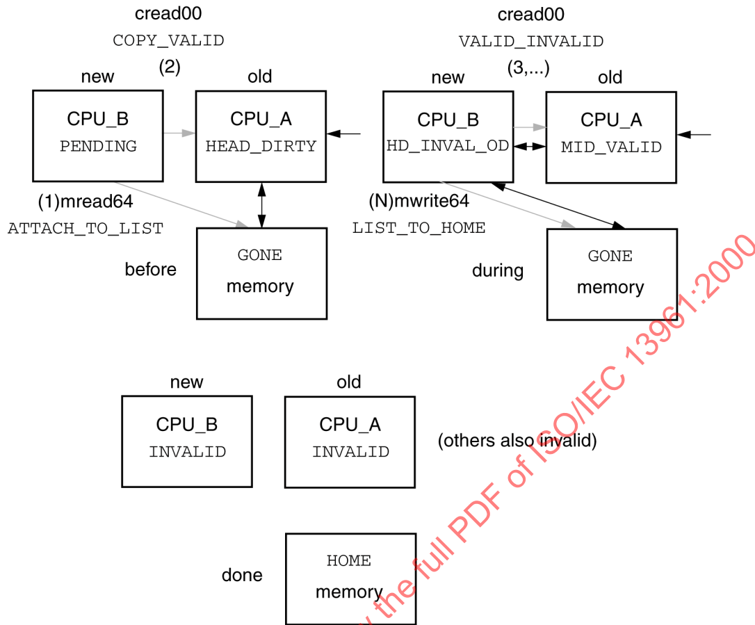
Figure 160 – Flushing a GONE list
