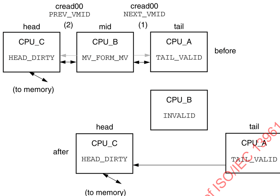
Figure 148 – Mid-entry deletions
