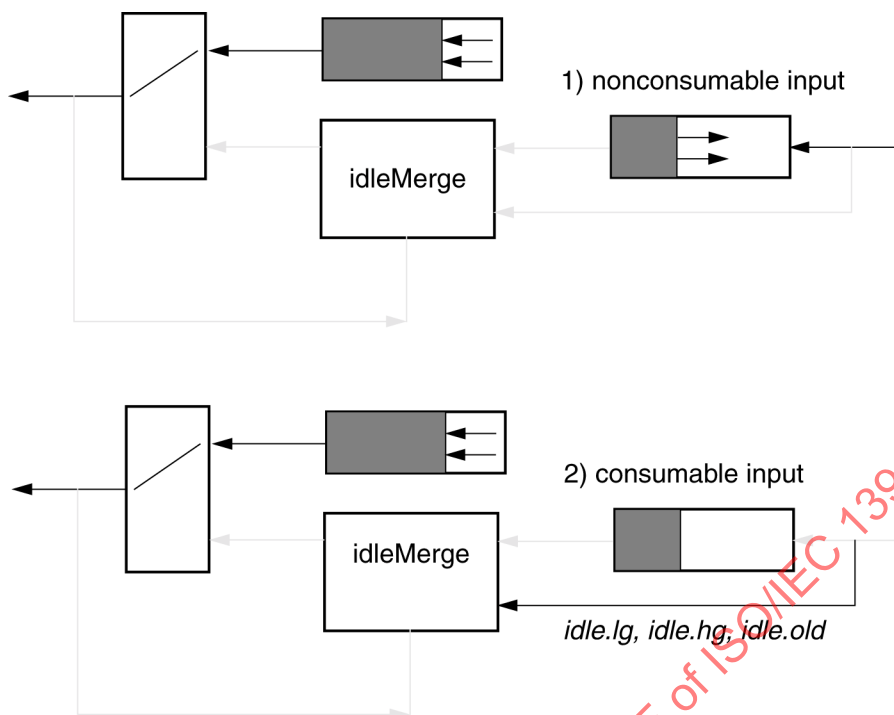
Figure 73 – Pass-transmission active
