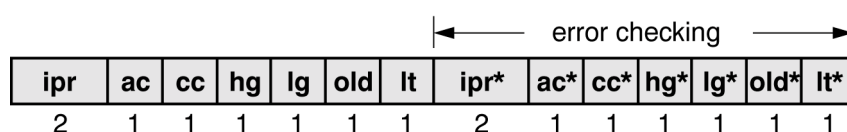
Figure 46 – Logical idle-symbol encoding
