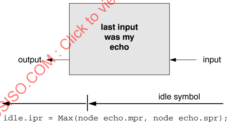
Figure 66 – Restoring ringlet priority
