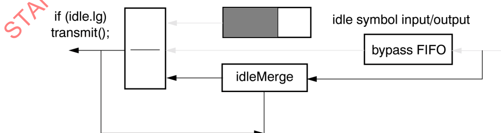
Figure 76 – Low-transmission enabled
