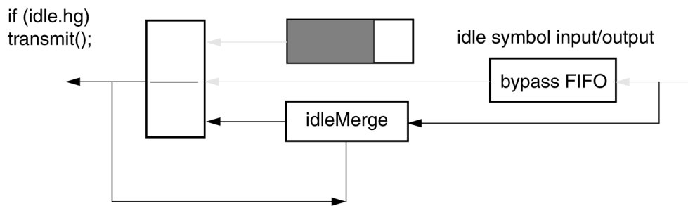
Figure 81 – High-transmission enabled
