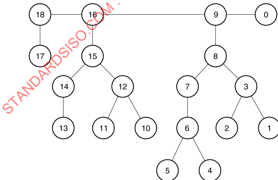
Figure 28 – Binary tree
