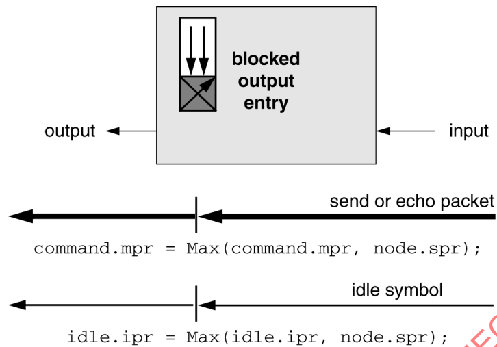
Figure 65 – Increasing ringlet priority
