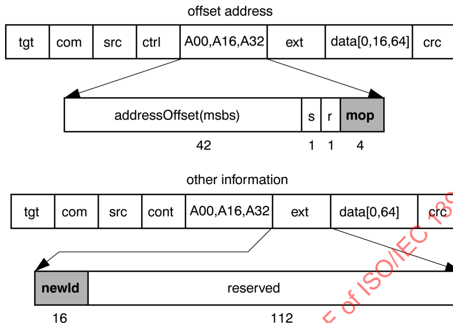
Figure 172 – Extended coherent memory read request
