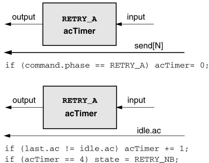
Figure 96 – Consumer error recovery
