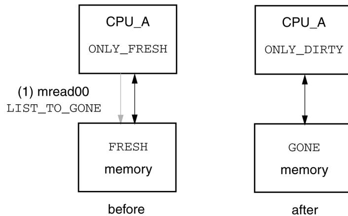
Figure 146 – ONLY_FRESH list conversion
