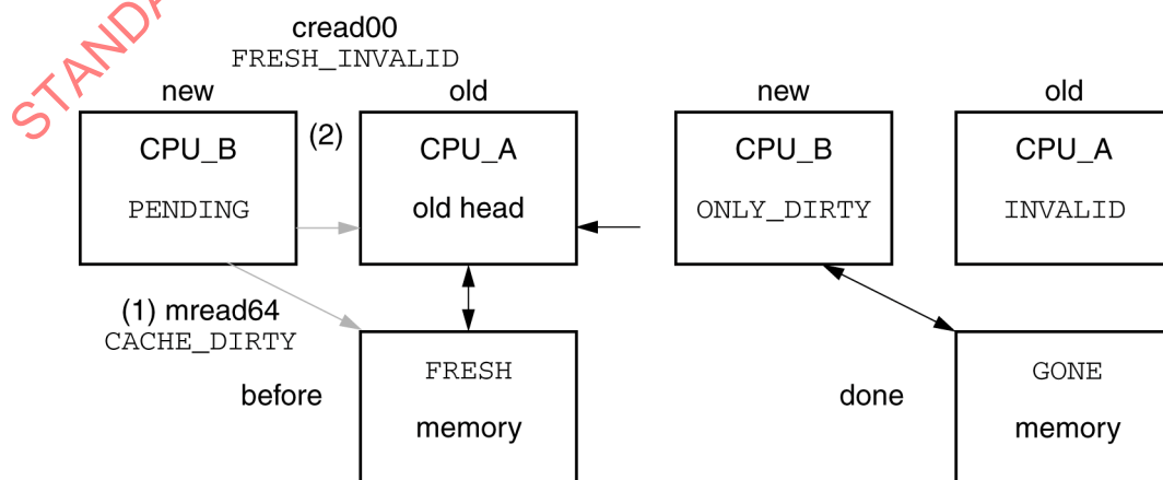
Figure 137 – FRESH list additions (minimal set)
