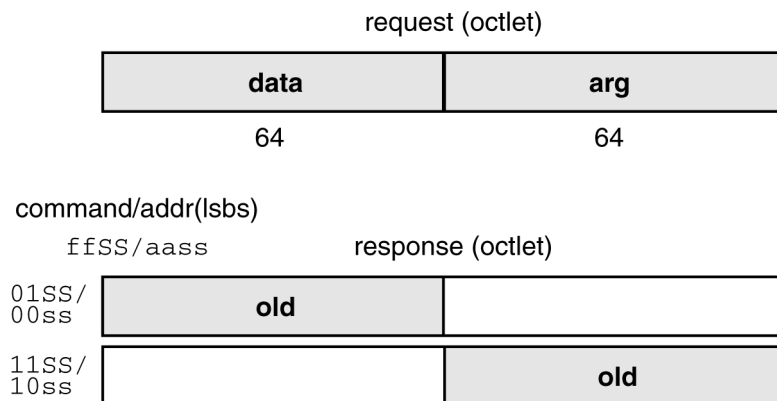
Figure 55 – Selected-byte locks (octlet access)
