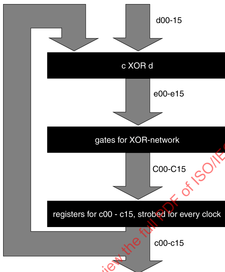
Figure 44 – Parallel CRC check
