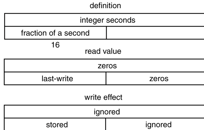
Figure 114 – SPLIT_TIMEOUT register-pair format
