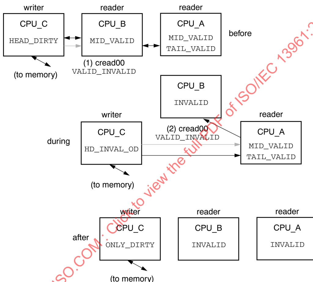
Figure 145 – Head purging others
