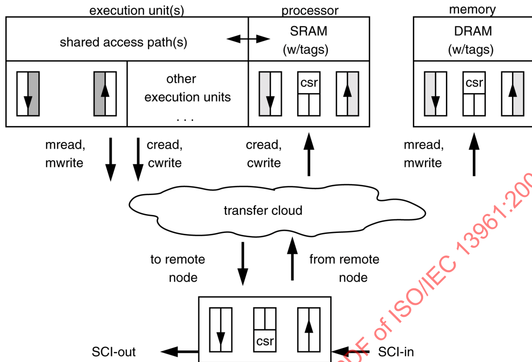
Figure 177 – One node's transfer-cloud model
