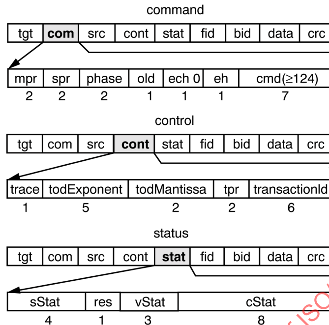
Figure 39 – Response-packet symbols
