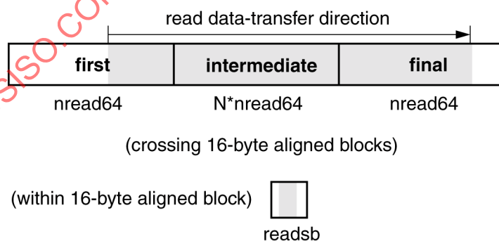
Figure 56 – Expected DMA read transfers
