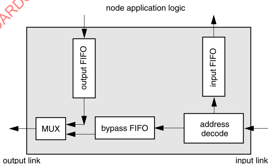
Figure 2 – SCI node model
