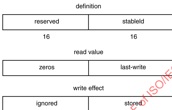
Figure 119 – SAVE_ID register (offset 520)
