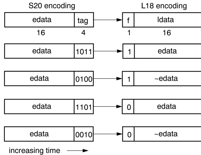
Figure 110 – S20 symbol decoding
