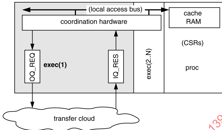
Figure 182 – An exec component's packet queues
