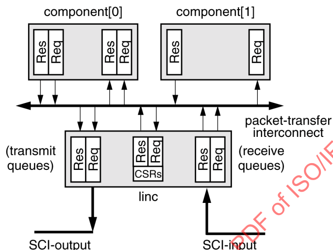
Figure 176 – Linc and component queues
