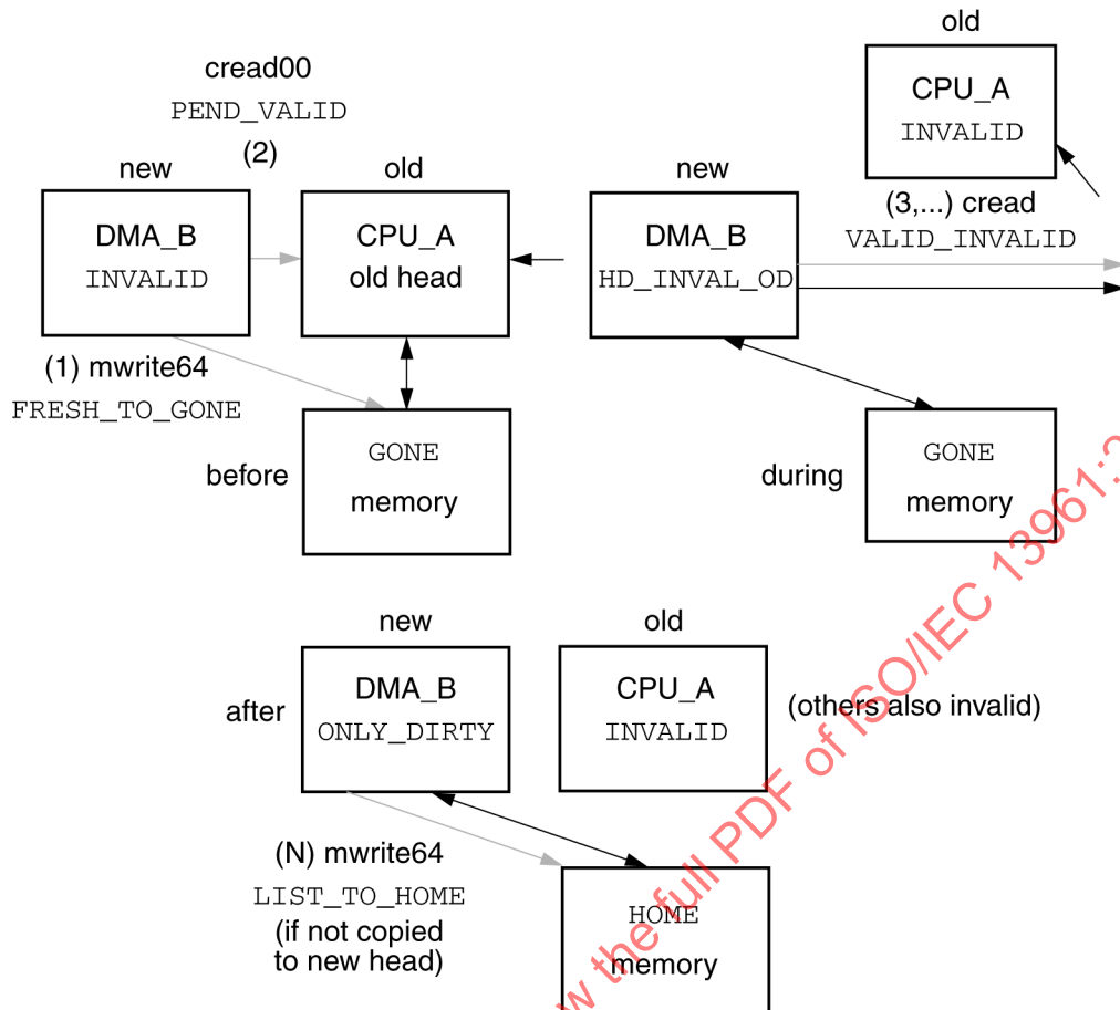
Figure 153 – Checked DMA write (memory GONE)
