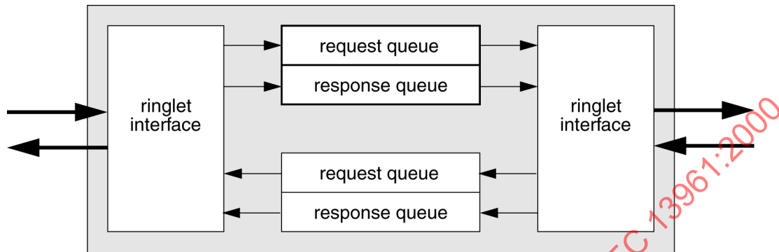
Figure 15 – Basic SCI bridge, paired request and response queues
