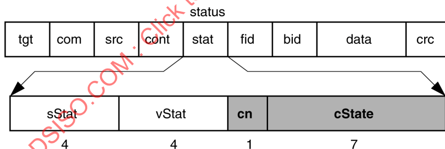
Figure 174 – Cache cread and cwrite64 responses
