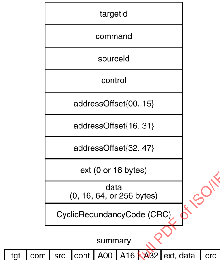
Figure 35 – Request-packet format
