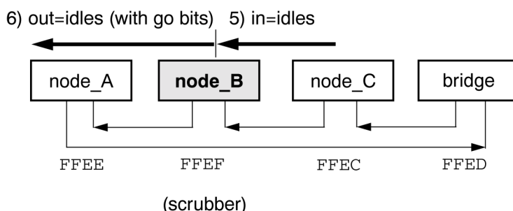
Figure 101 – Idle-closure injects go-bits in idles
