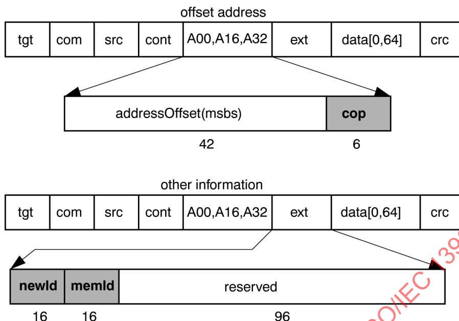
Figure 173 – Cache cread and cwrite64 requests
