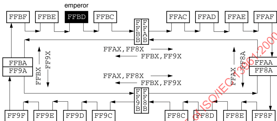
Figure 107 – Nodelds after emperor selection, final address assignments
