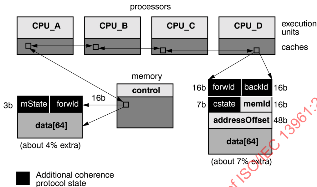
Figure 130 – SCI coherence tags (64-byte line, 64K nodes)
