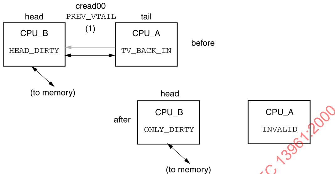
Figure 139 – Tail-entry deletions
