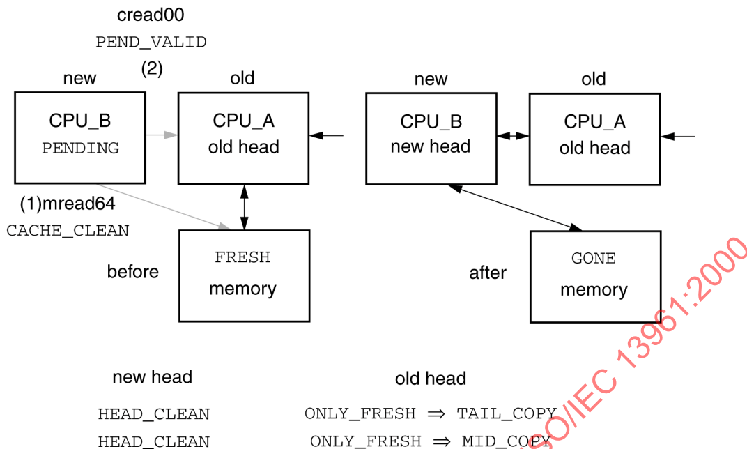
Figure 156 – CLEAN addition to FRESH list
