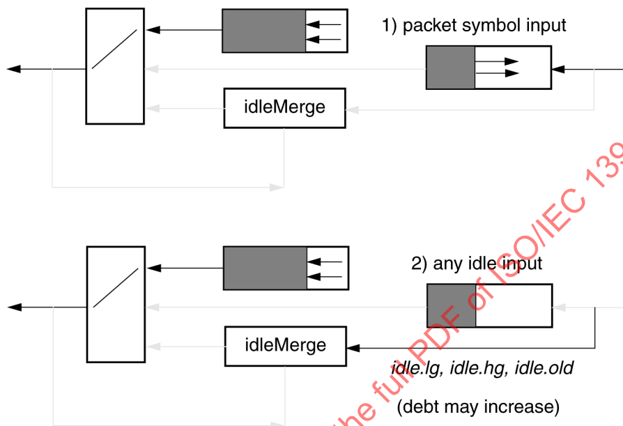
Figure 77 – Low-transmission active
