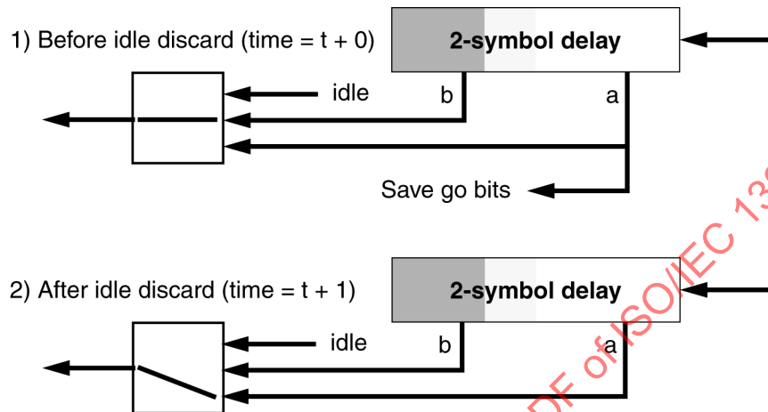
Figure 63 – Idle-symbol deletion
