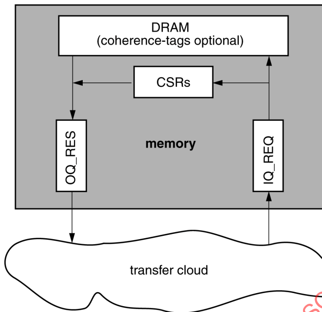
Figure 181 – A memory component's packet queues
