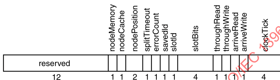
Figure 122 – ROM format, CsrOptions
