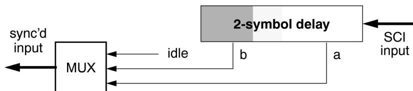
Figure 61 – Input-synchronizer model
