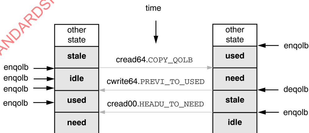
Figure 169 – QOLB usage
