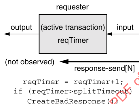
Figure 84 – Response timeouts (request and no response)
