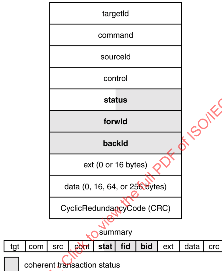
Figure 38 – Response-packet format
