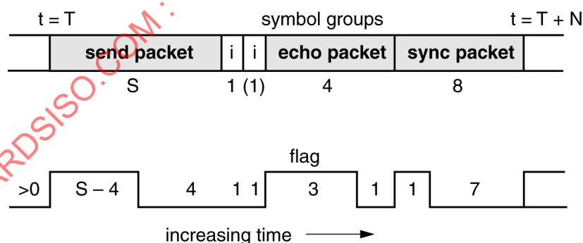
Figure 47 – Flag framing convention
