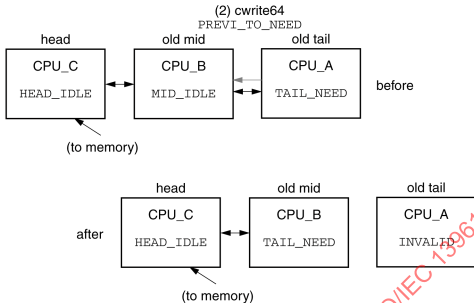
Figure 168 – Deqolb tail-deletion on QOLB sharing list
