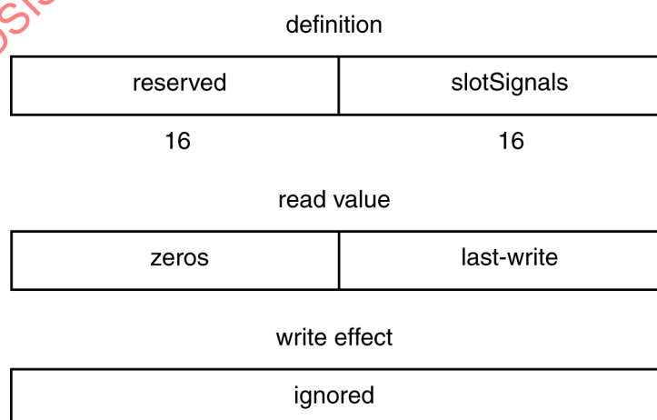
Figure 120 – SLOT_ID register (offset 524)
