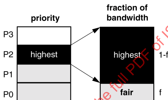
Figure 23 – Bandwidth partitioning
