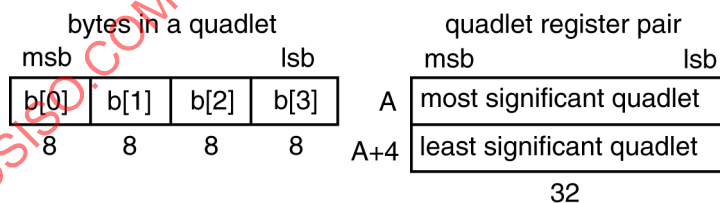
Figure 33 – Big-endian register notation
