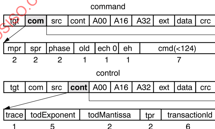
Figure 36 – Request-packet symbols
