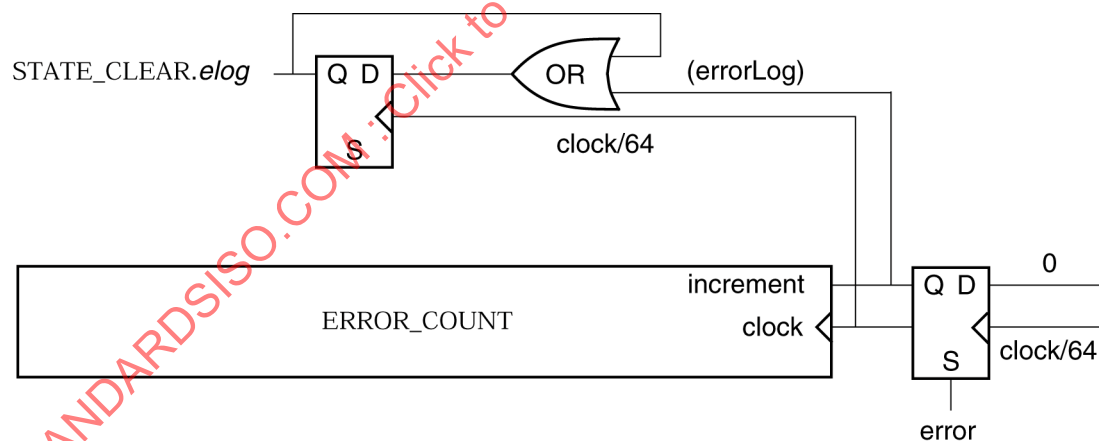
Figure 90 – Error-logging registers
