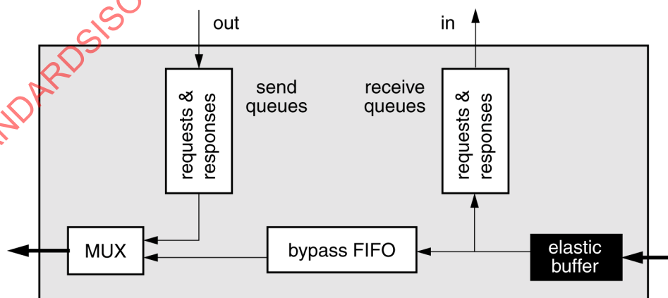
Figure 60 – Elasticity model
