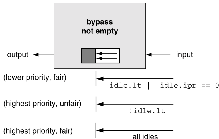
Figure 70 – Idle consumption, unfair-capable node
