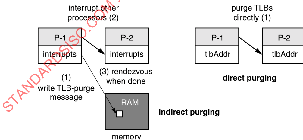
Figure 29 – TLB purging
