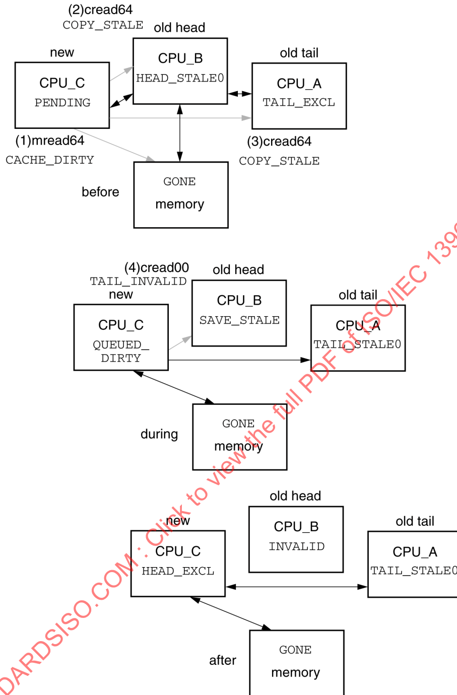
Figure 164 – Prepending to pairwise list (HEAD_STALE0)
