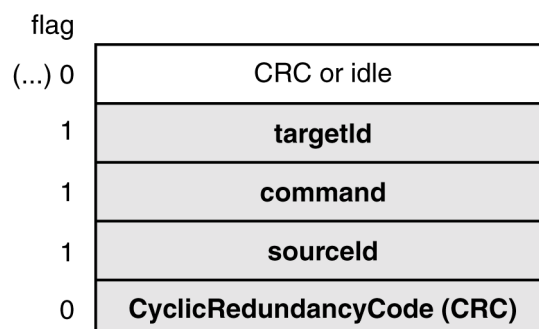
Figure 49 – Logical echo-packet framing convention
