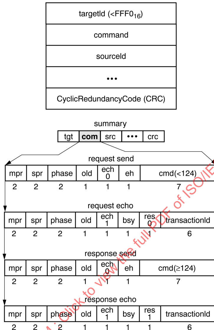
Figure 34 – Send- and echo-packet formats
