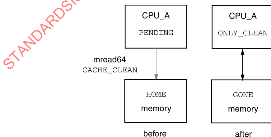
Figure 154 – CLEAN list creation
