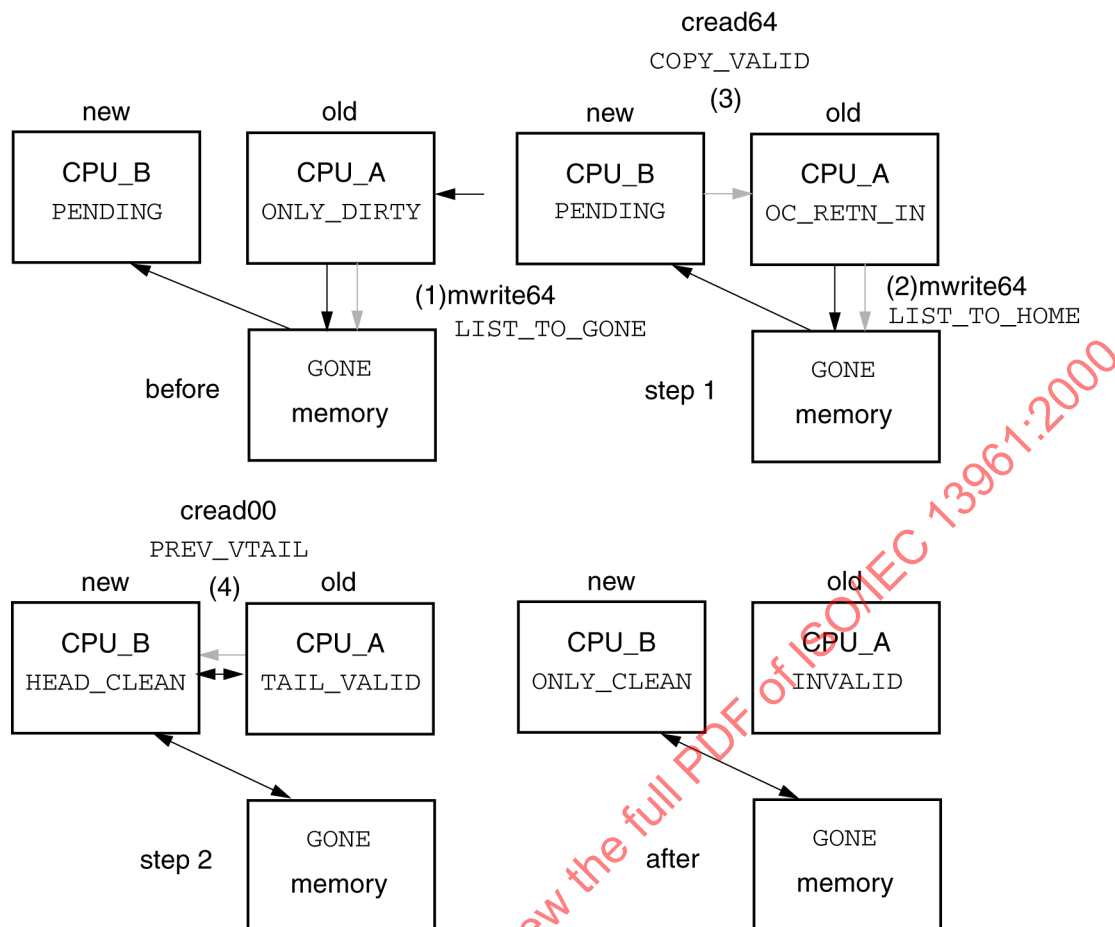
Figure 161 – Cleansing DIRTY sharing lists (prepend conflict)
