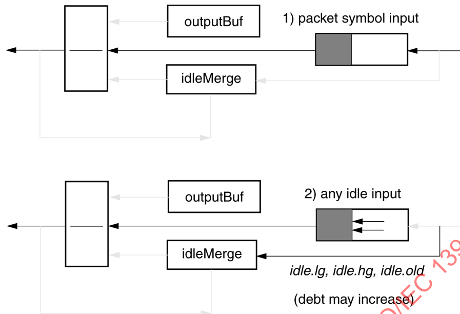
Figure 78 – Low/high-transmission recovery
