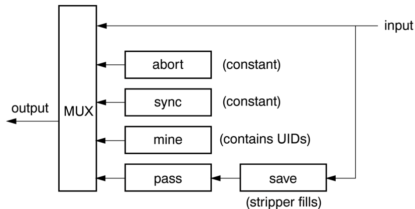
Figure 105 – Insert-multiplexer model
