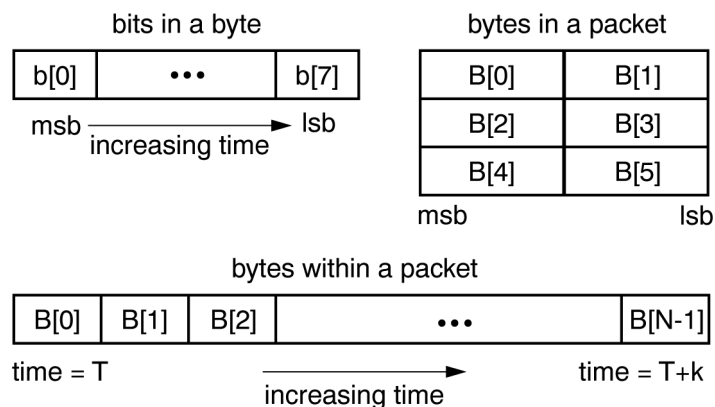
Figure 32 – Big-endian packet notation
