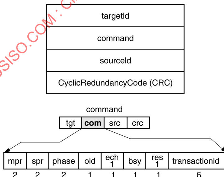
Figure 40 – Response-echo packet format
