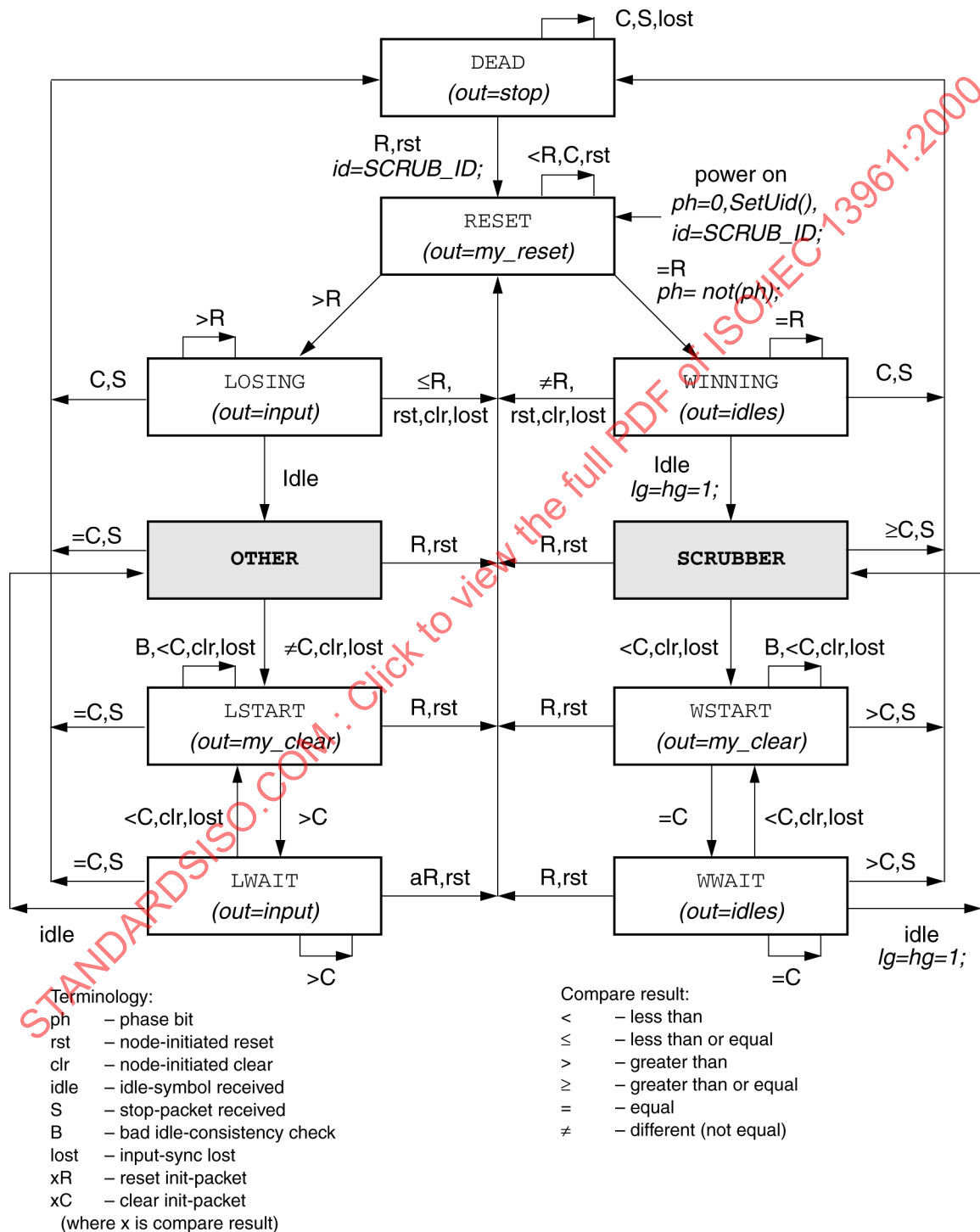
Figure 103 – Initialization states (clear option)
