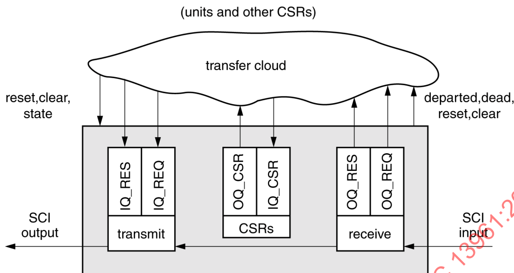
Figure 178 – The linc packet queues
