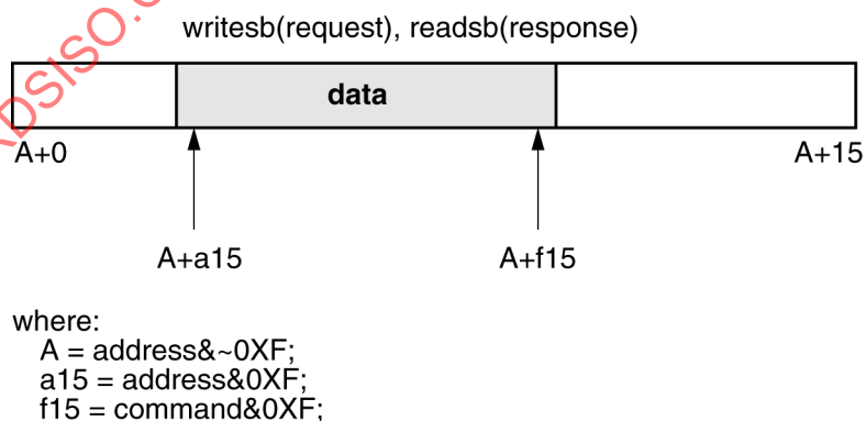
Figure 52 – Selected-byte reads and writes
