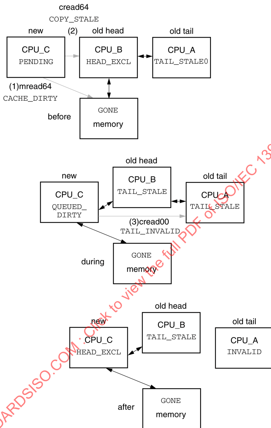
Figure 163 – Prepending to pairwise list (HEAD_EXCL)
