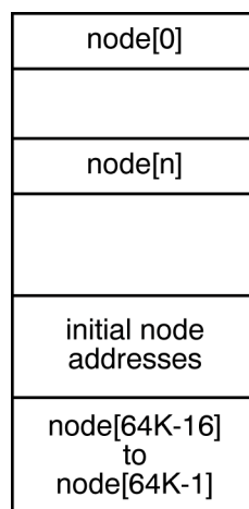
Figure 97 – SCI (64-bit fixed) addressing
