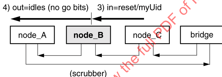
Figure 100 – Reset-closure generates idle symbols
