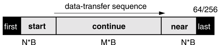
Figure 58 – DMA block-transfer model
