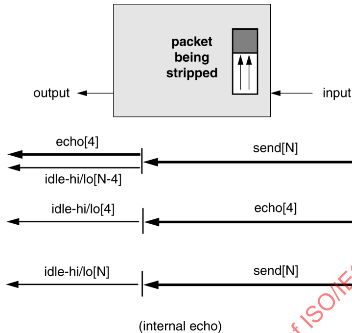
Figure 68 – Idle-symbol creation, unfair-capable node
