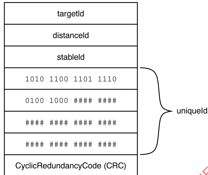
Figure 42 – Initialization-packet format example ( companyId -based uniqueId value)
