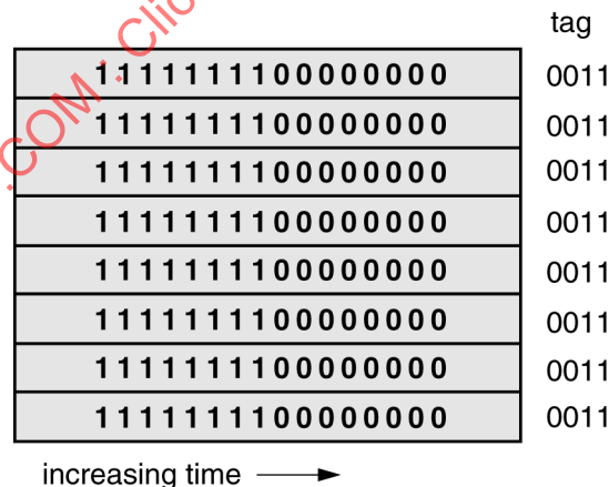
Figure 111 – S20 sync-packet encoding
