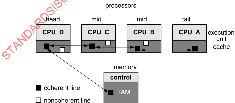
Figure 26 – Distributed cache tags
