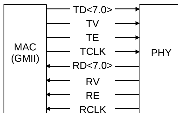
Figure 2 – MAC interface
