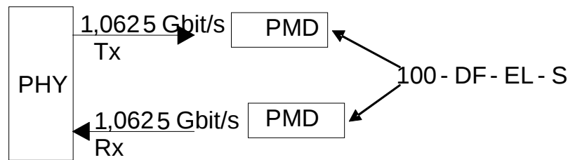
Figure 3 – Interface overview via 100 Ω Class F cabling
