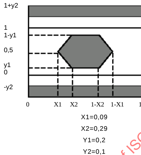
Figure 10 – Transmission eye diagram
