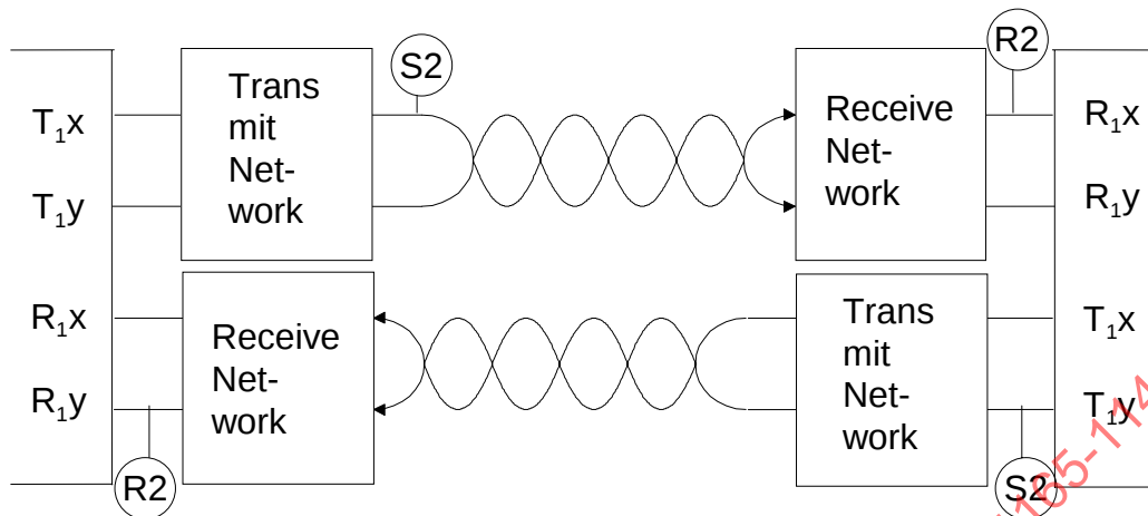
Figure 7 – Transmission with MLT-3
