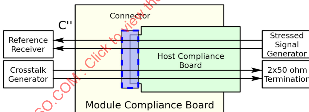
Figure 7 – Host input calibration point C''
