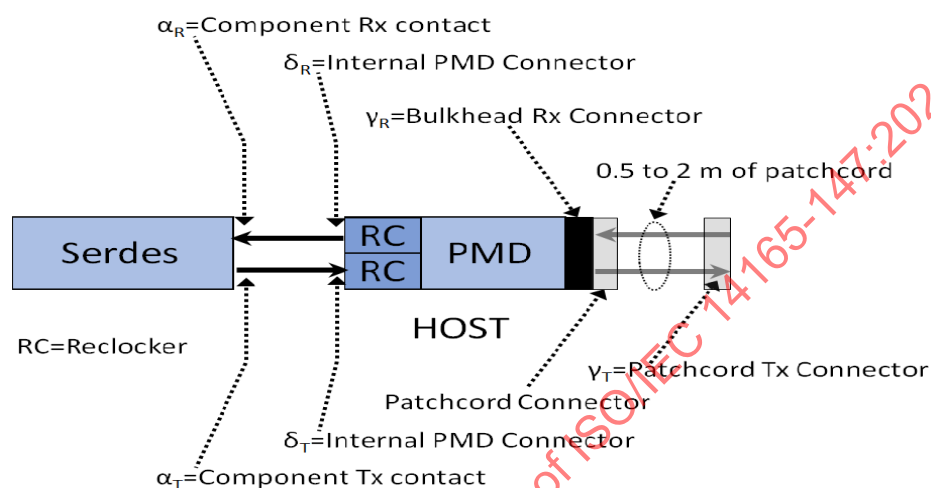
Figure 2 – Compliance points for 64GFC PMDs
