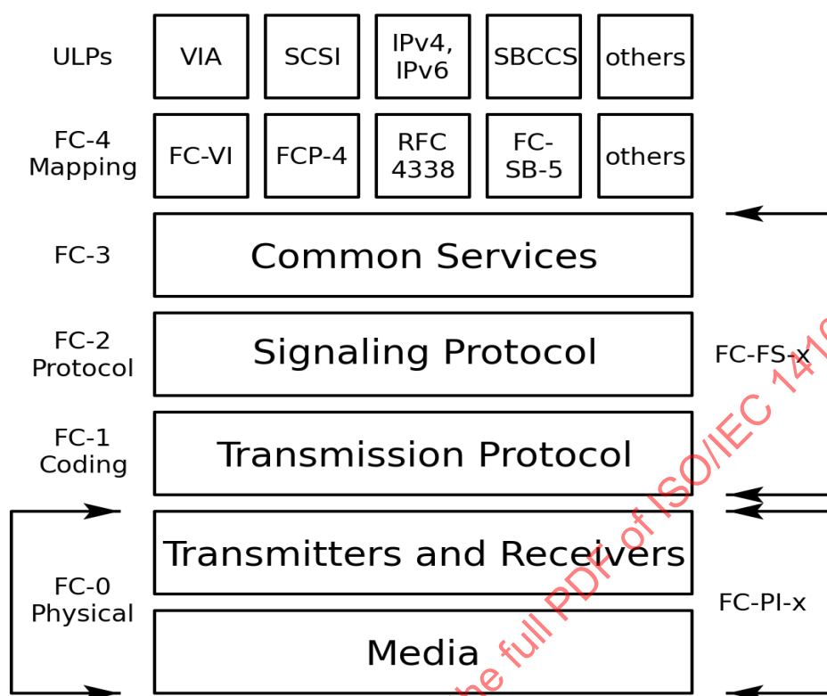
Figure 1 – Fibre Channel hierarchy
