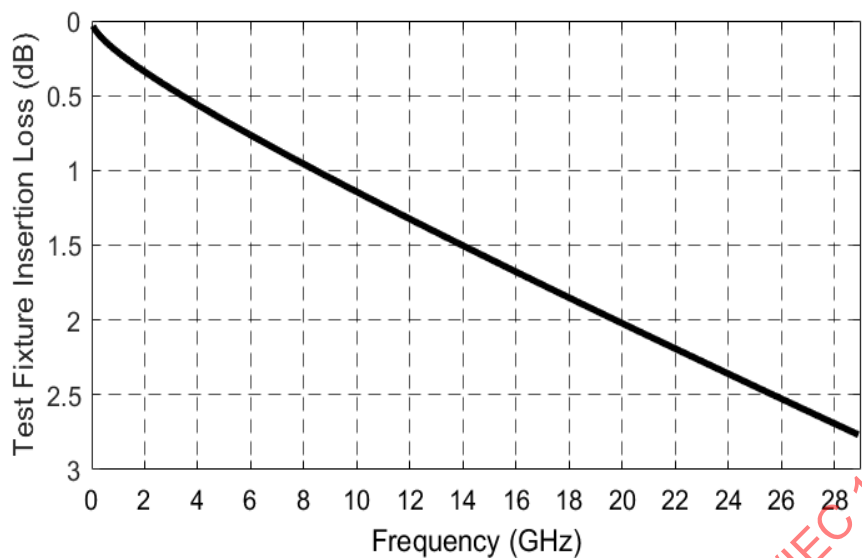
Figure 12 – Test fixture reference insertion loss
