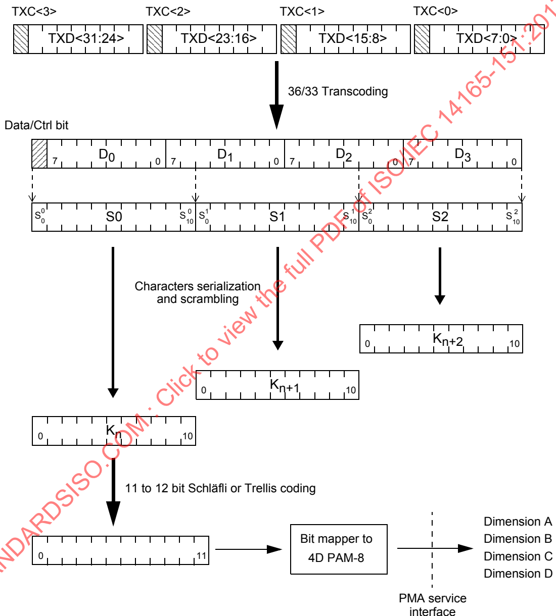
Figure 9 – PCS transmit bit ordering
