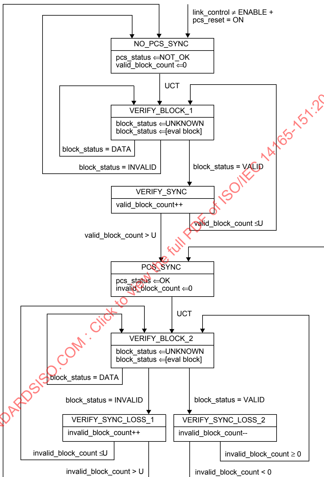
Figure 19 – PCS synchronization state diagram
