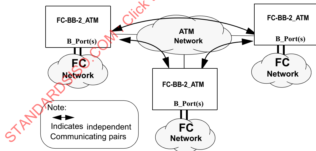
Figure 2 – FC-BB-2_ATM Reference Model
