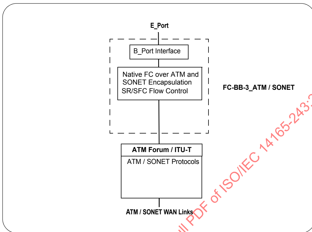
Figure 1 – Scope and components of FC-BB-3_ATM/SONET models
