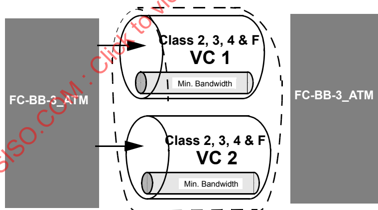
Figure 18 – Recommended ATM bandwidth allocation for multiple VCs
