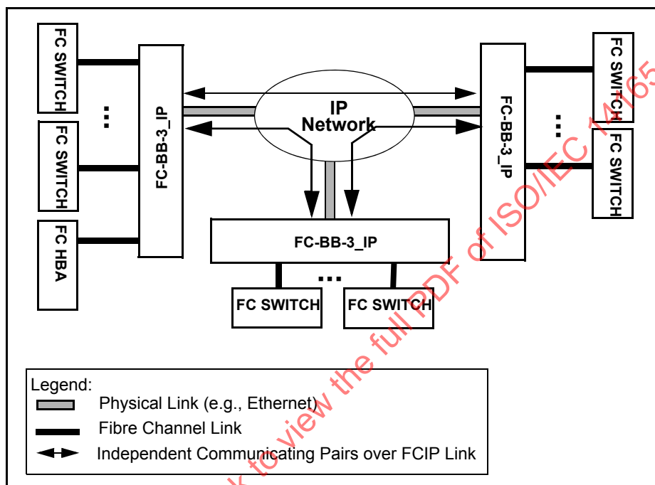
Figure 25 – FC-BB-3_IP network configuration
