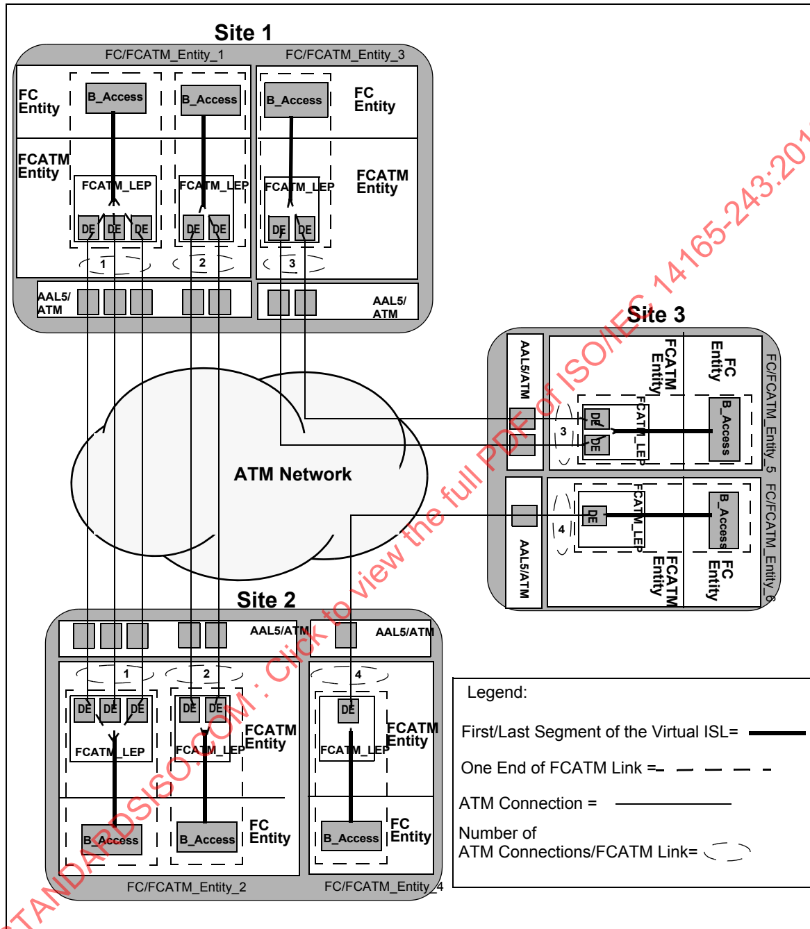
Figure 15 – FC-BB-3_ATM network topologies
