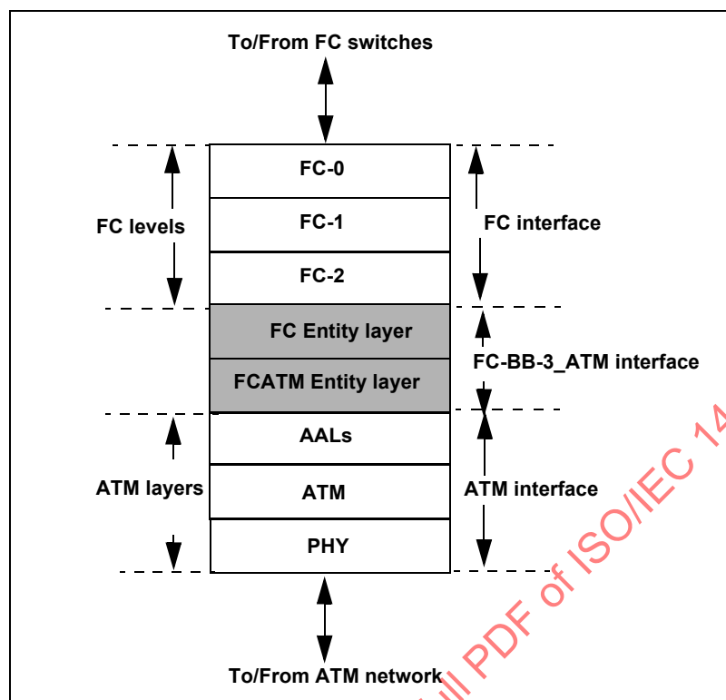
Figure 10 – FC-BB-3_ATM protocol layers
