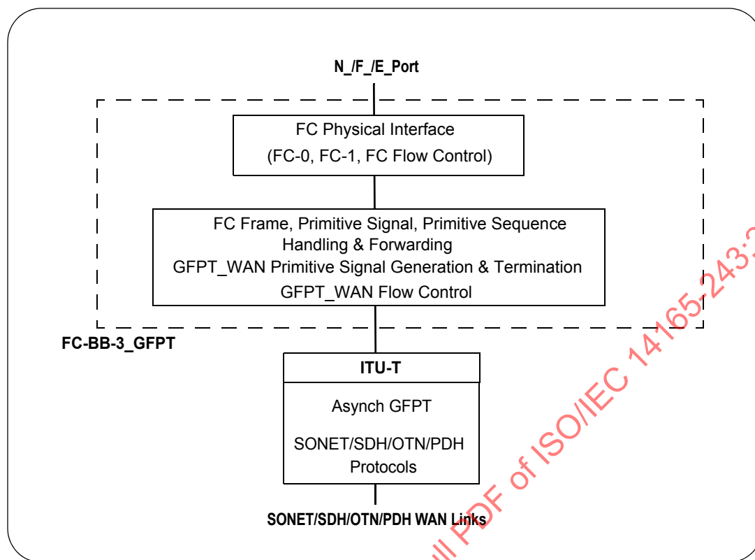
Figure 3 – Scope and components of FC-BB-3_GFPT model
