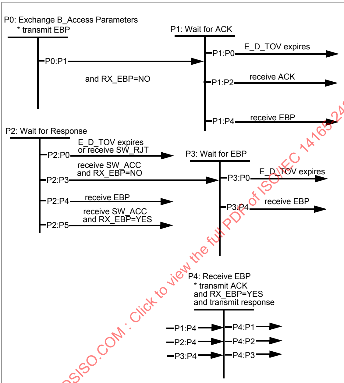
Figure 14 – B_Access initialization state machine
