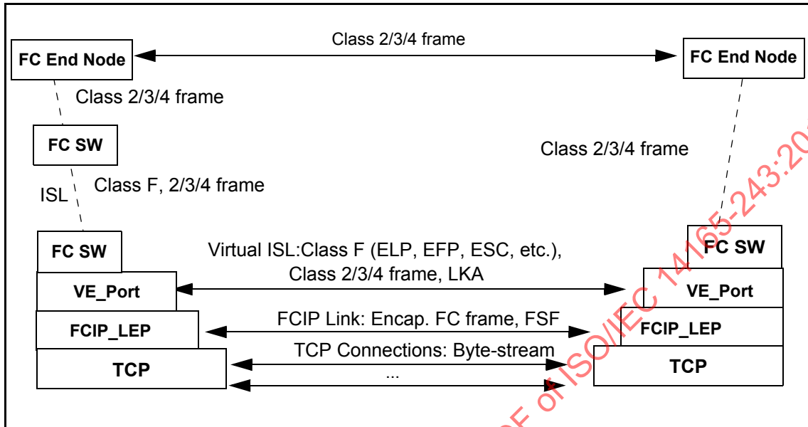
Figure 28 – Scope of VE_Port Virtual ISL
