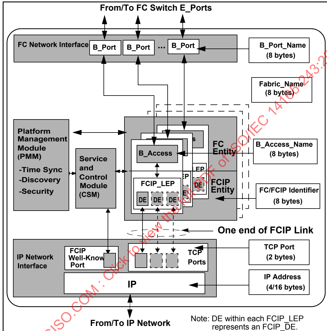
Figure 30 – FC-BB-3_IP B_Access functional model
