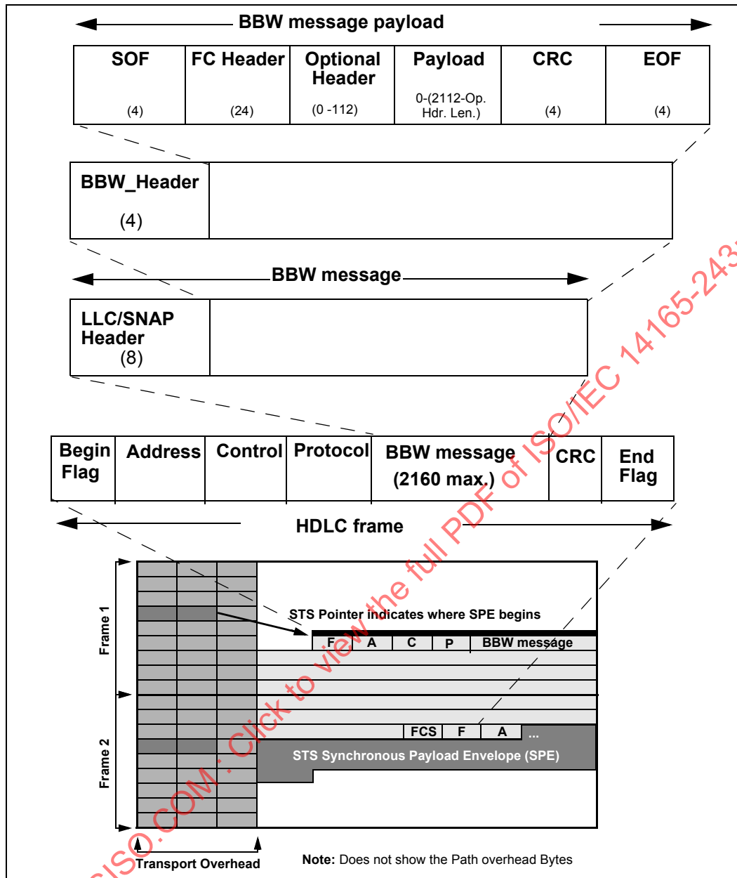
Figure 23 – Encapsulation of BBW message into HDLC frame using SFC
