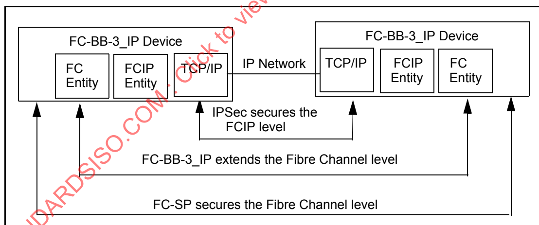
Figure 29 – Security layers
