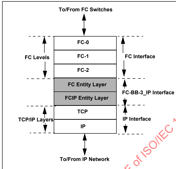
Figure 27 – FC-BB-3_IP Protocol Layers
