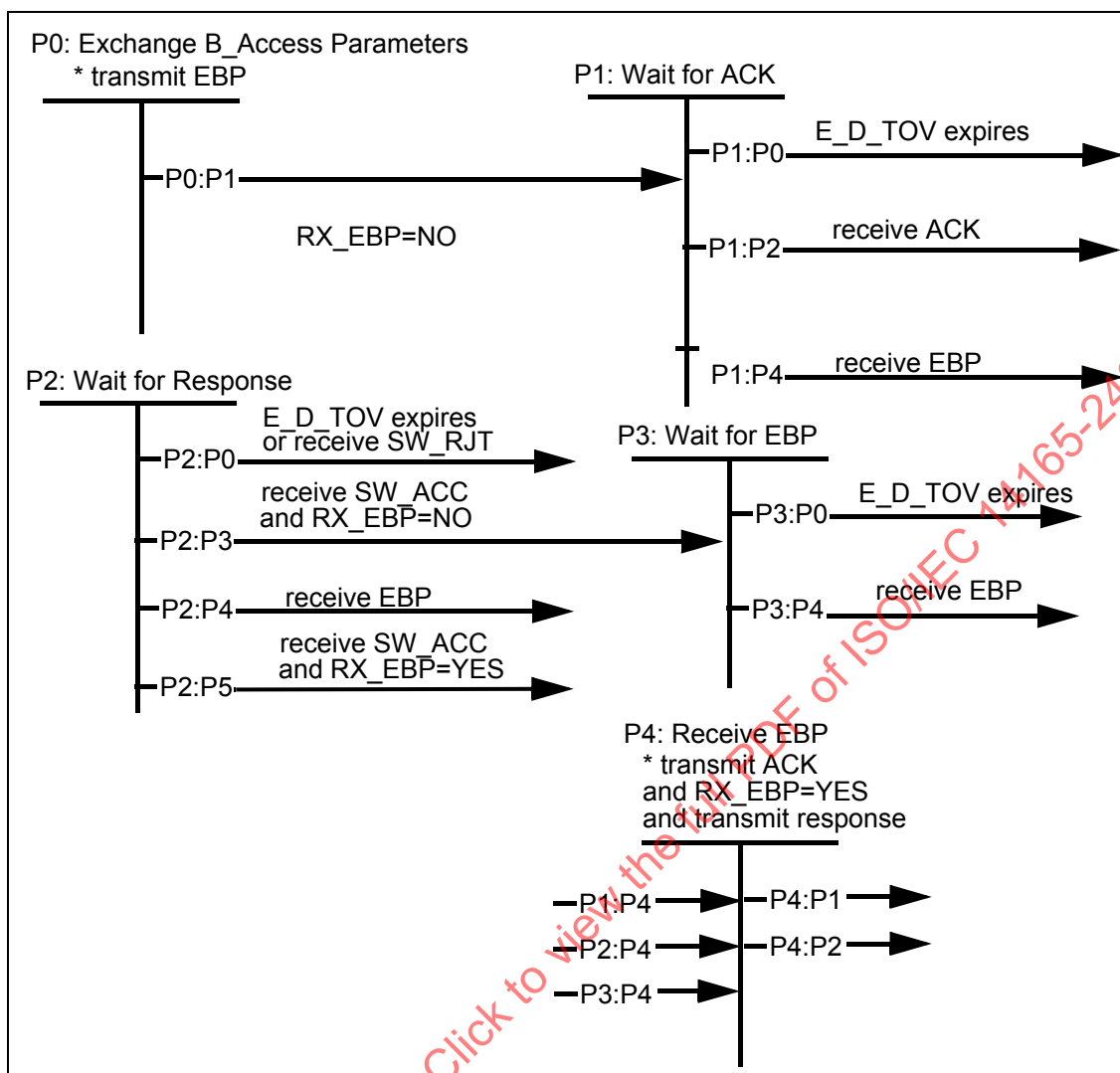
Figure 32 – B_Access initialization state machine
