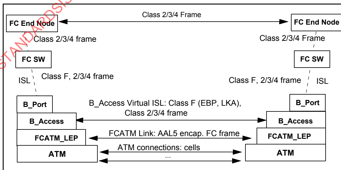
Figure 13 – Scope of B_Access Virtual ISL
