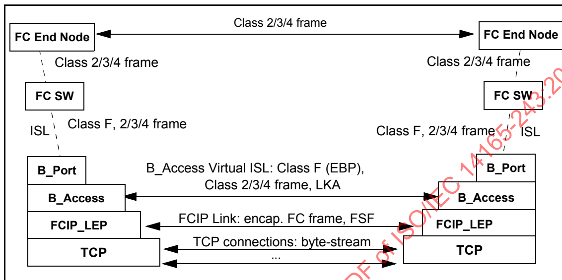
Figure 31 – Scope of B_Access Virtual ISL
