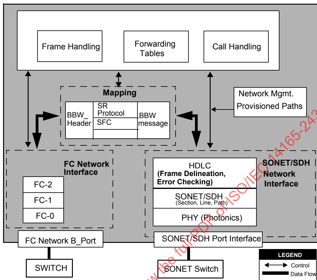
Figure 20 – FC-BB-3_SONET functional block diagram
