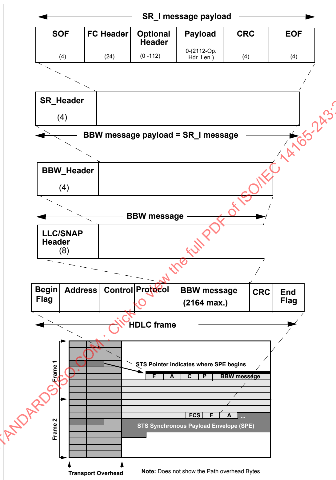
Figure 24 – Encapsulation of BBW message into HDLC frame using SR
