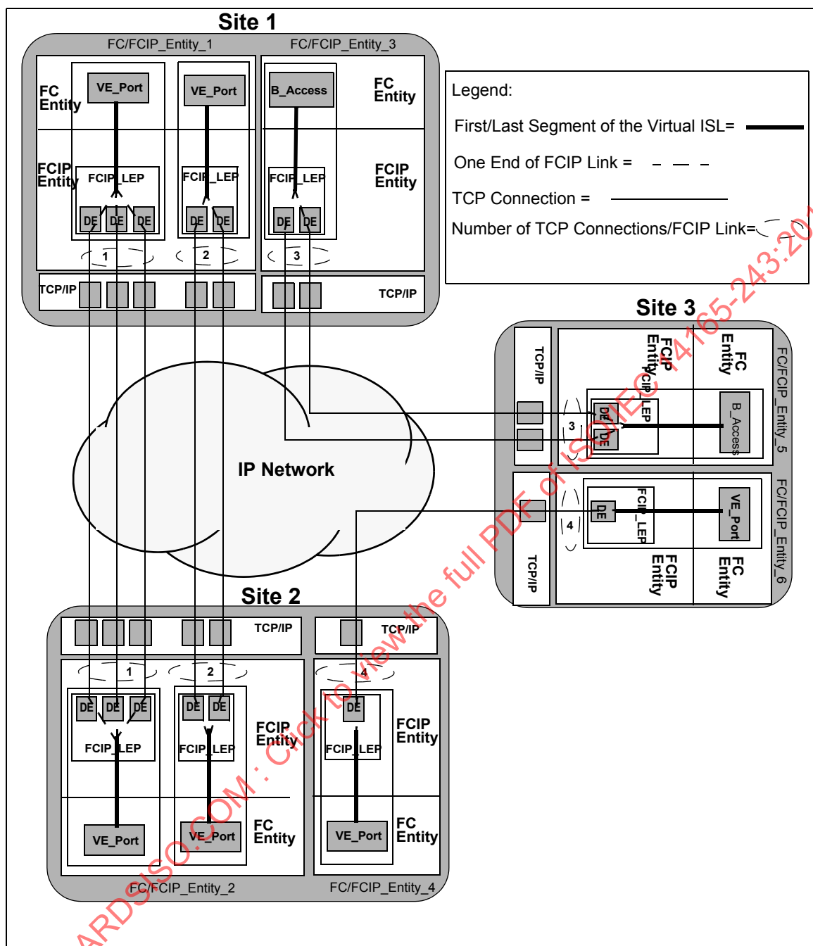
Figure 33 – FC-BB-3_IP network topologies
