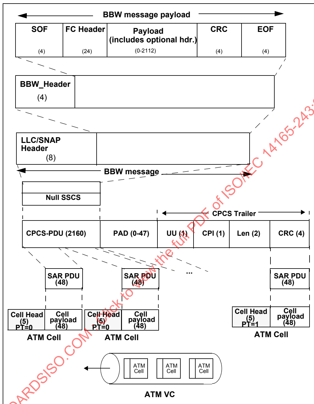
Figure 16 – AAL5 Mapping of a BBW message with SFC
