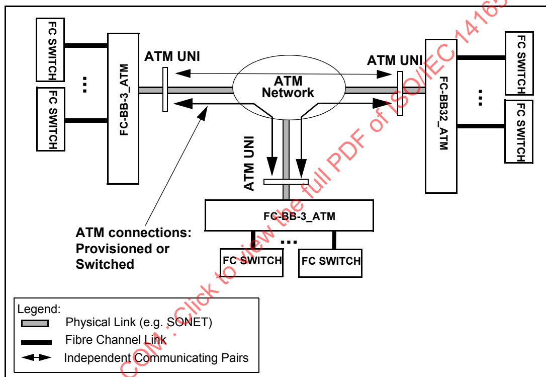
Figure 9 – FC-BB-3_ATM network configuration
