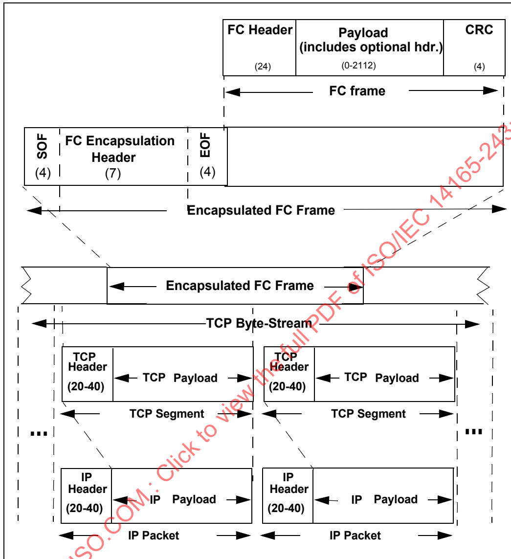
Figure 34 – TCP/IP encapsulation of an encapsulated FC frame
