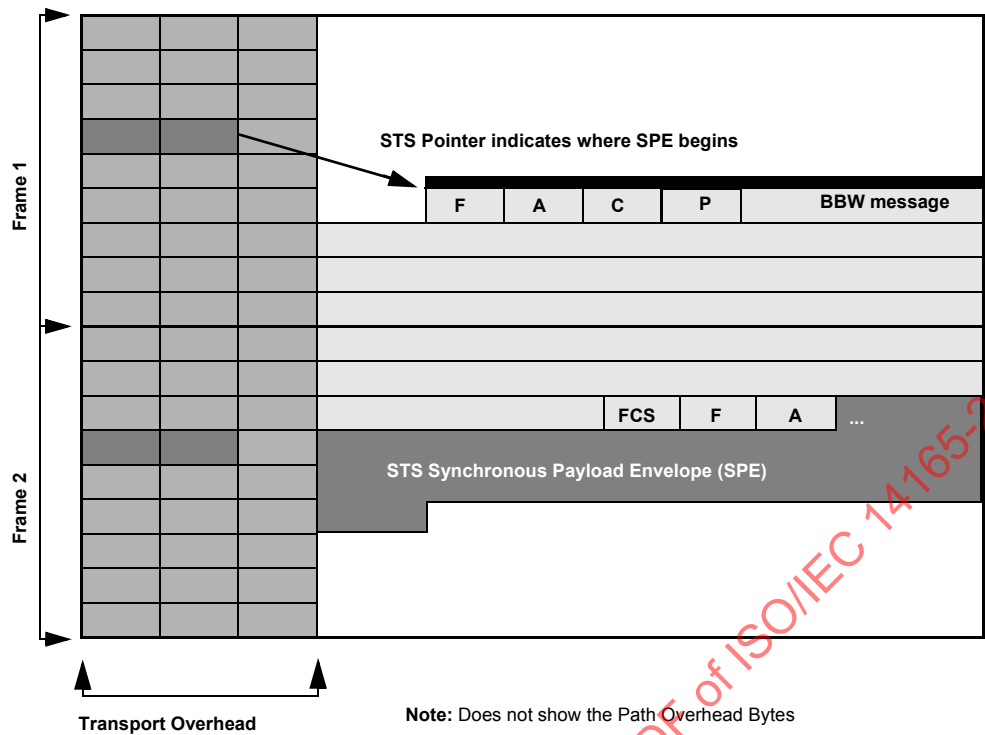
Figure 21 – SNET SPE HDLC mapping example
