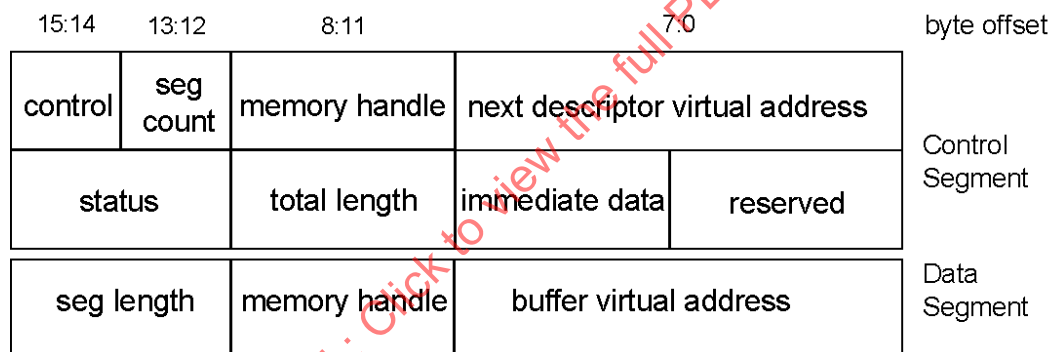
Figure 7: Send and Receive Descriptor Format
