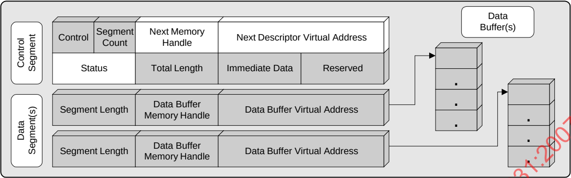
Figure 7: Descriptor fields updated by VI Application
