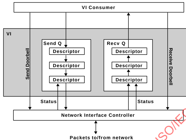
Figure 2: A Virtual Interface
