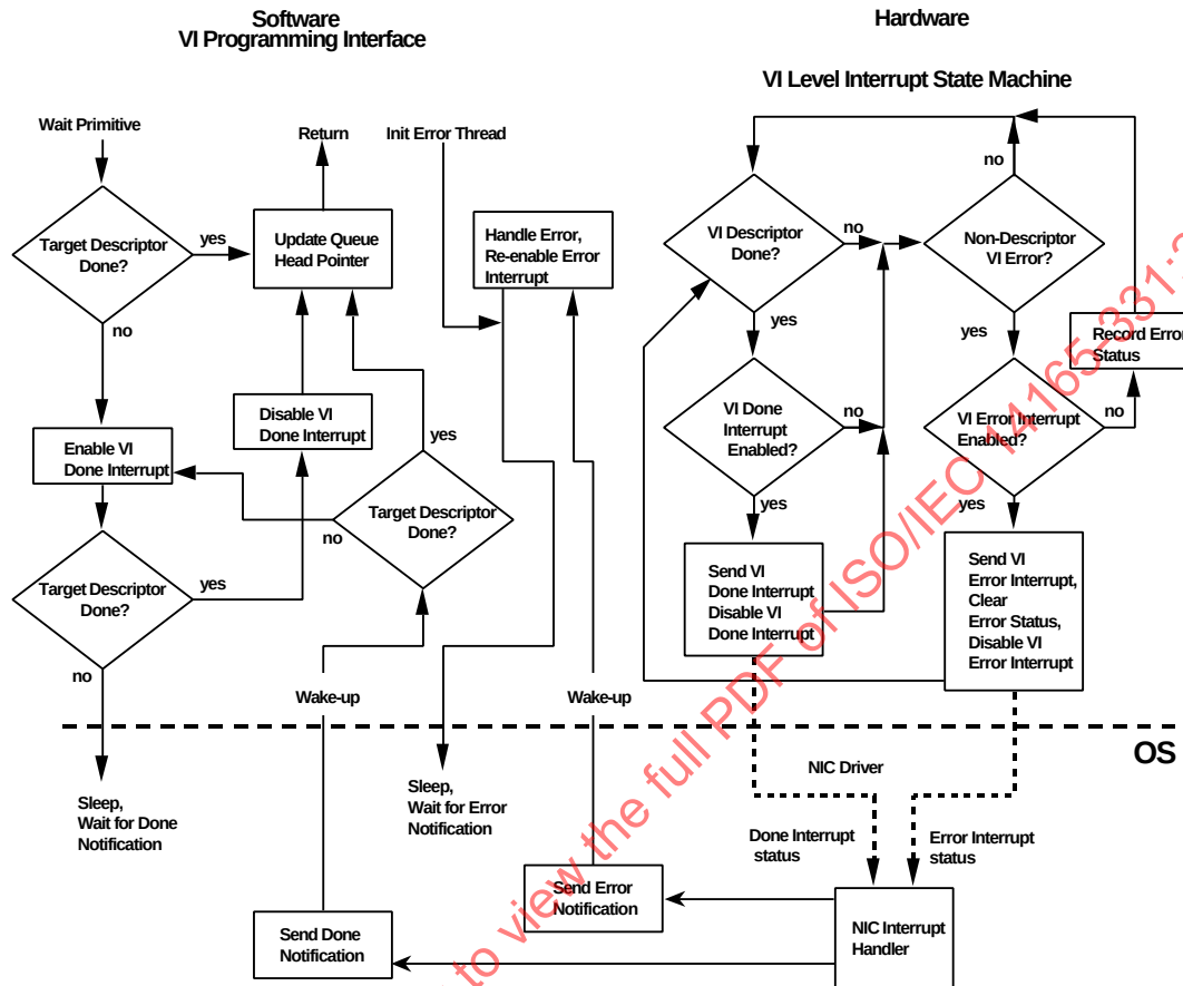
Figure 12: Asynchronous Event Model
