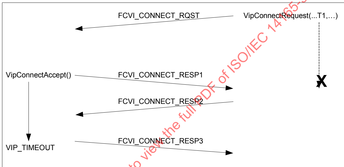
Figure C.2 – Client timeout of VipConnectRequest
