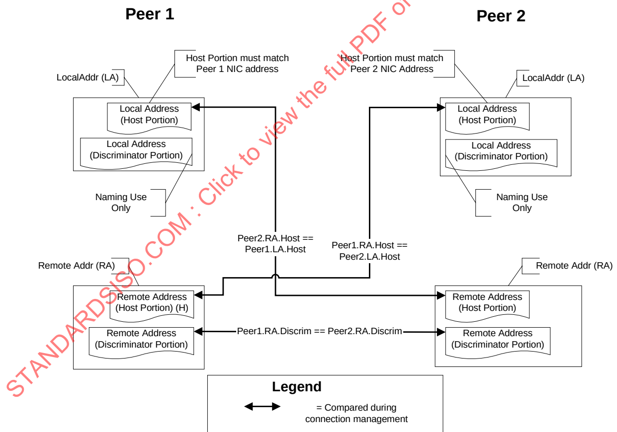
Figure 11: Address Comparison and Data Exchange for Peer-to-Peer
