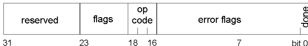
Figure 9: Status Field Format
