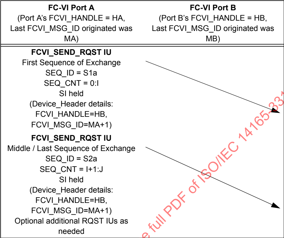
Figure 2 – FC-VI send for Unreliable Delivery or Reliable Delivery
